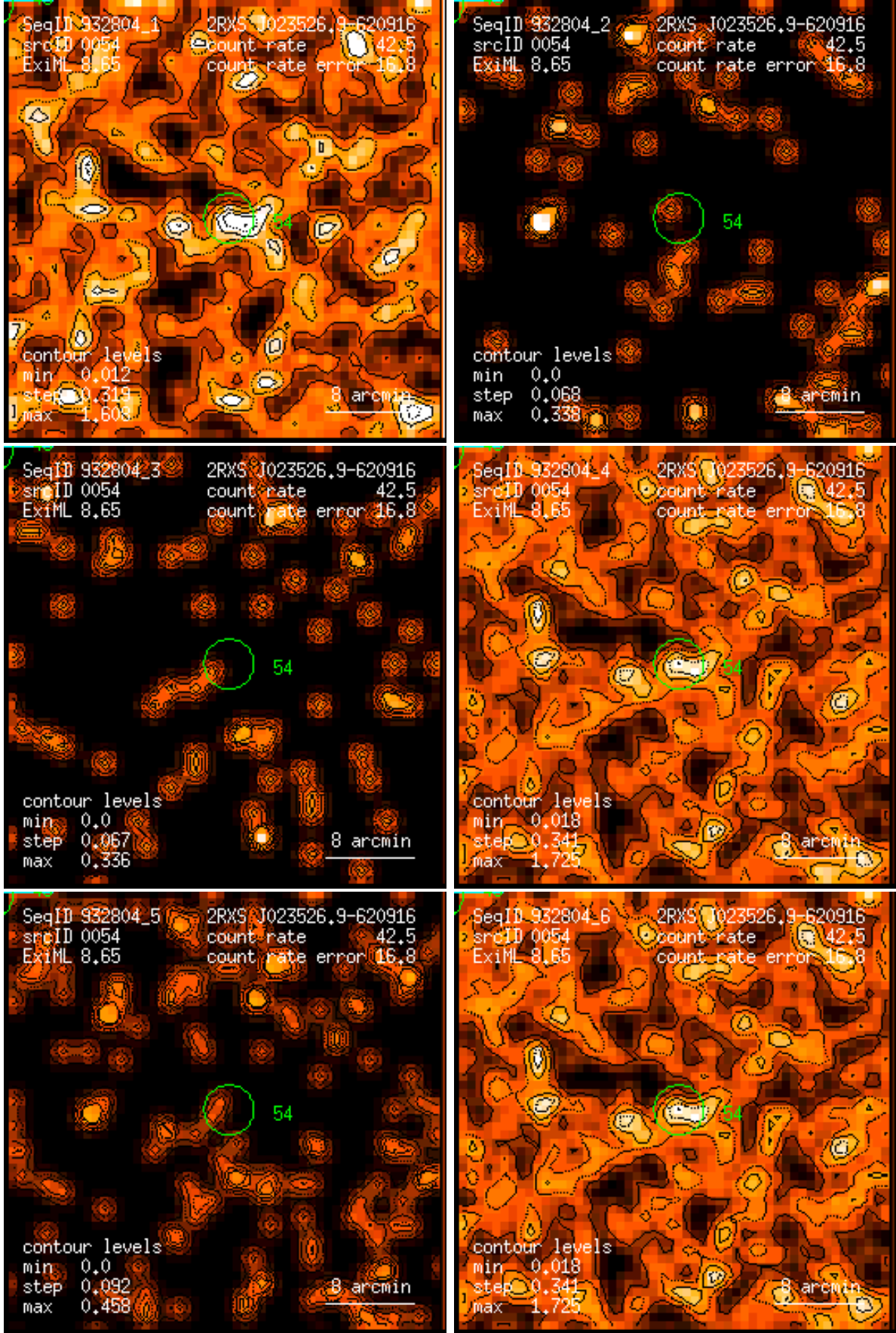
Figure 54: RASS 932804: detection 0054: band rate images, Gaussian filter: (1) PSPC channels 11 – 41, (2) 52 – 90, (3) 91 – 201, (4) 11 – 235, (5) 52 – 201, (6) 11 – 201. Broad band rates in counts/ks. Band rate contour levels in counts/ks/arcmin 2 .
