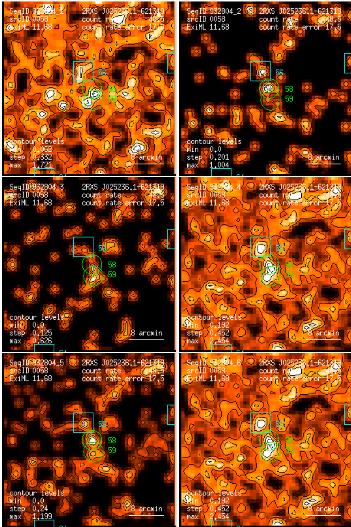
Figure 58: RASS 932804: detection 0058: band rate images, Gaussian filter: (1) PSPC channels 11 – 41, (2) 52 – 90, (3) 91 – 201, (4) 11 – 235, (5) 52 – 201, (6) 11 – 201. Broad band rates in counts/ks. Band rate contour levels in counts/ks/arcmin 2 .
