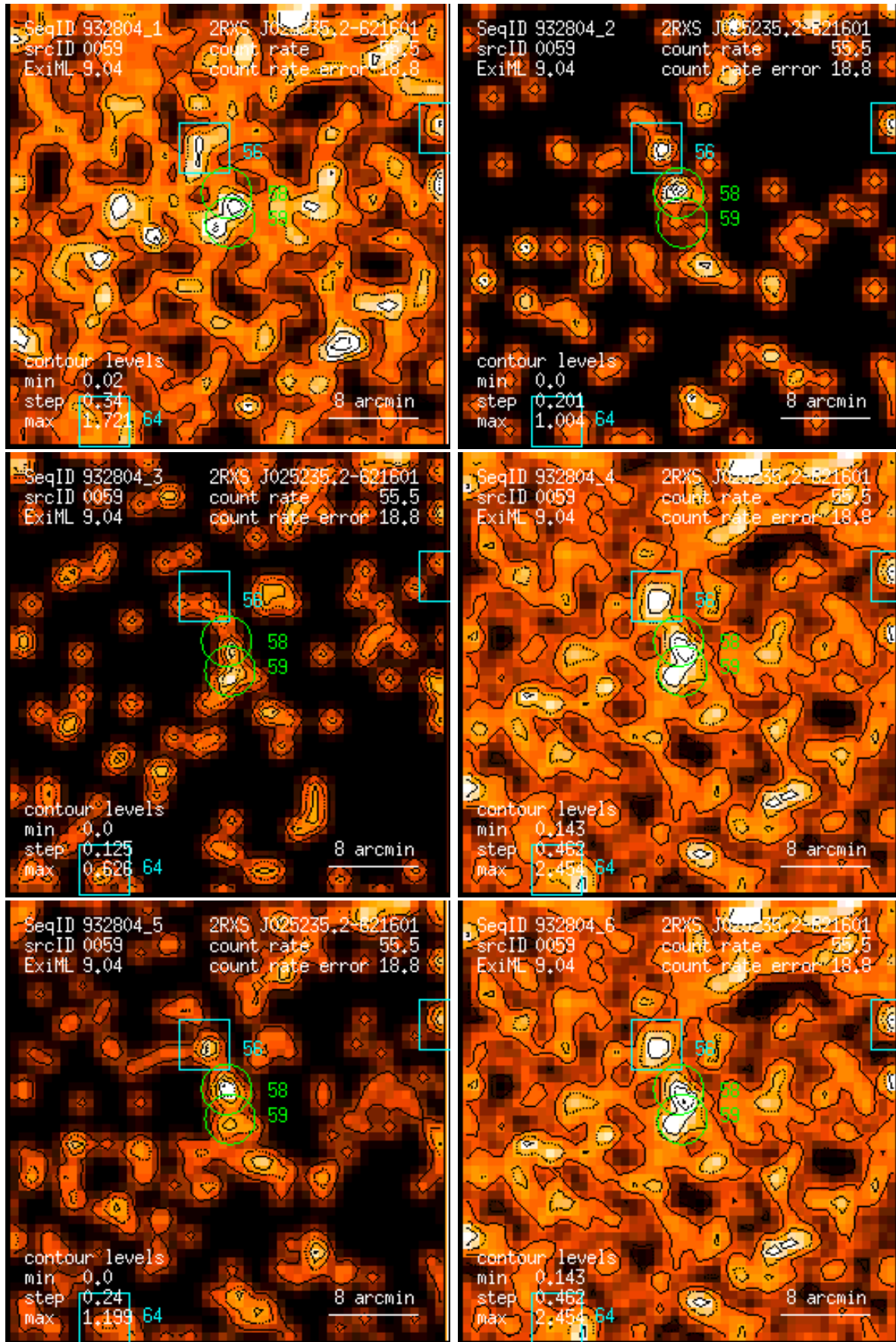
Figure 59: RASS 932804: detection 0059: band rate images, Gaussian filter: (1) PSPC channels 11 – 41, (2) 52 – 90, (3) 91 – 201, (4) 11 – 235, (5) 52 – 201, (6) 11 – 201. Broad band rates in counts/ks. Band rate contour levels in counts/ks/arcmin 2 .
