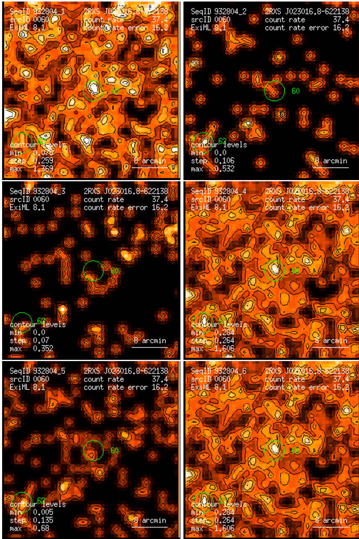
Figure 60: RASS 932804: detection 0060: band rate images, Gaussian filter: (1) PSPC channels 11 – 41, (2) 52 – 90, (3) 91 – 201, (4) 11 – 235, (5) 52 – 201, (6) 11 – 201. Broad band rates in counts/ks. Band rate contour levels in counts/ks/arcmin 2 .
