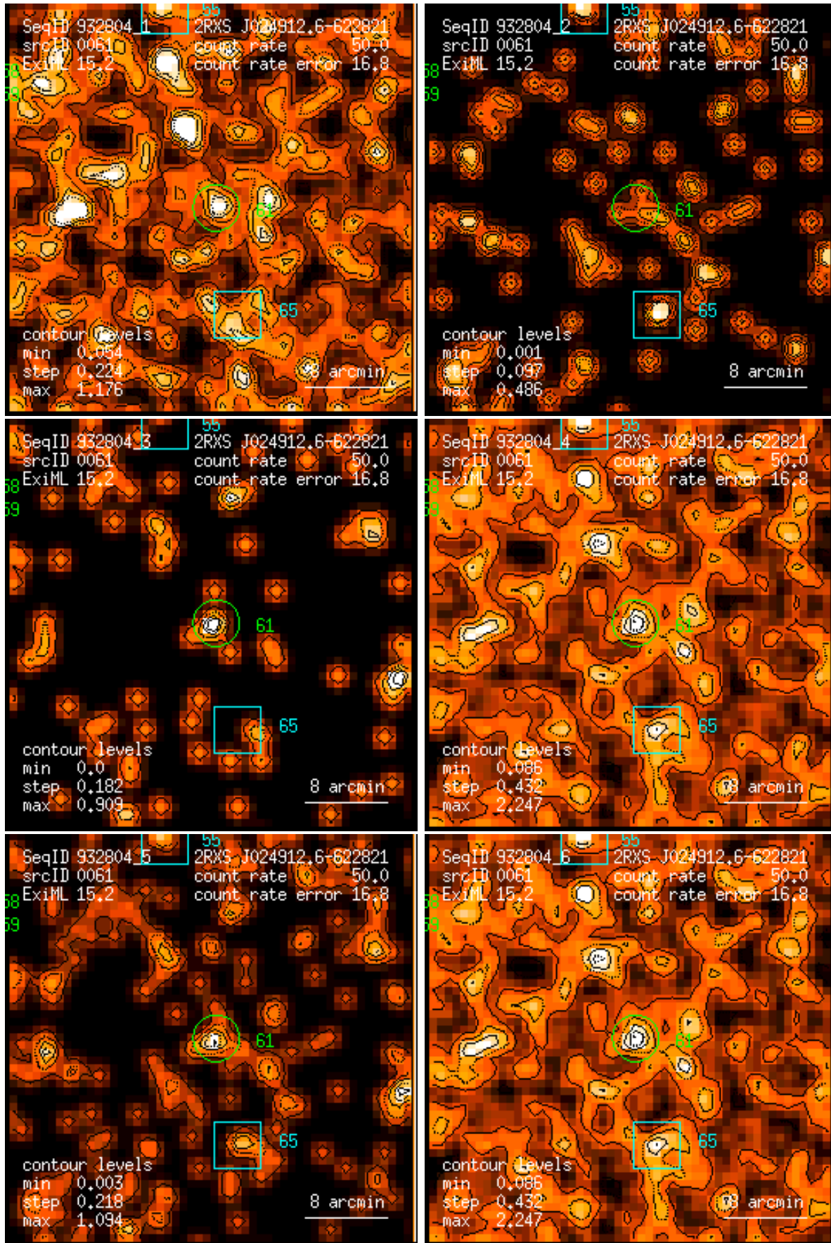
Figure 61: RASS 932804: detection 0061: band rate images, Gaussian filter: (1) PSPC channels 11 – 41, (2) 52 – 90, (3) 91 – 201, (4) 11 – 235, (5) 52 – 201, (6) 11 – 201. Broad band rates in counts/ks. Band rate contour levels in counts/ks/arcmin 2 .
