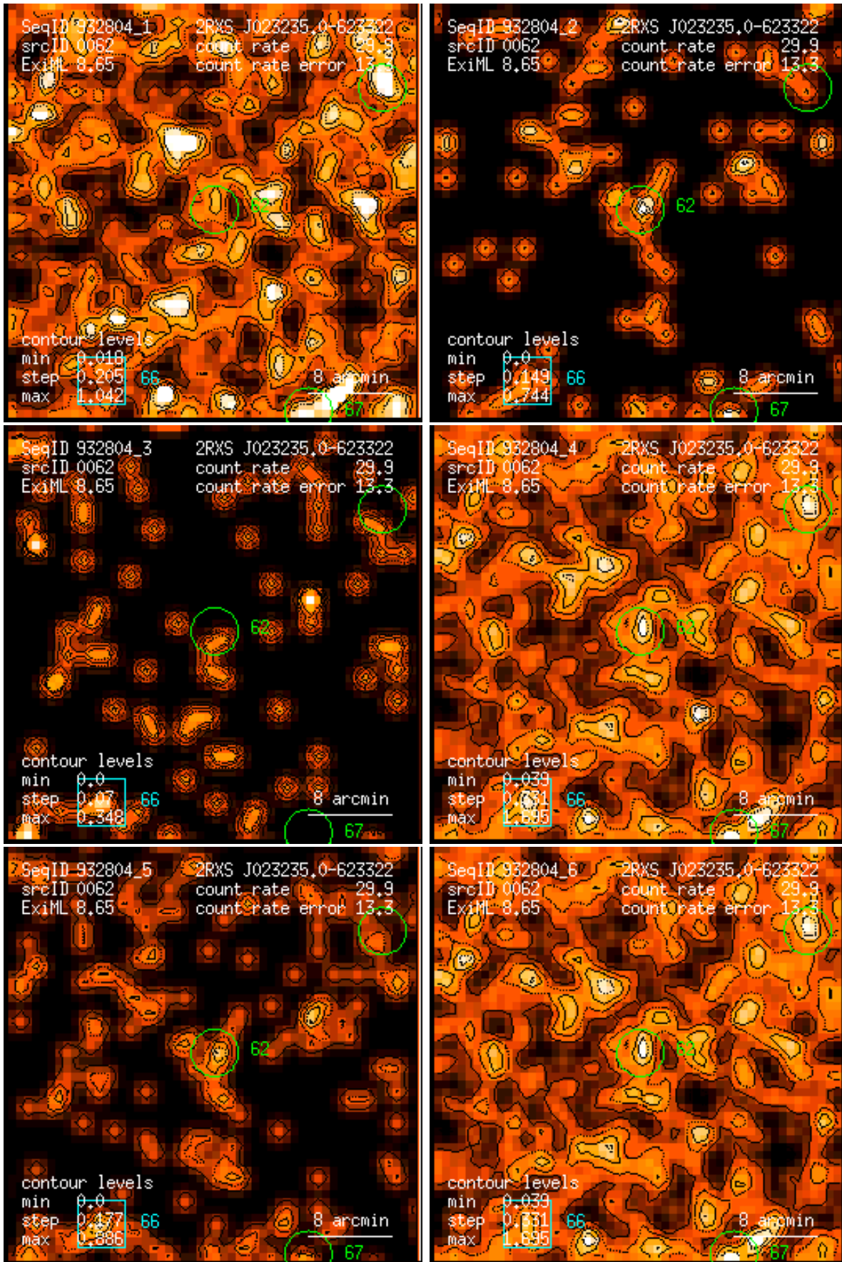
Figure 62: RASS 932804: detection 0062: band rate images, Gaussian filter: (1) PSPC channels 11 – 41, (2) 52 – 90, (3) 91 – 201, (4) 11 – 235, (5) 52 – 201, (6) 11 – 201. Broad band rates in counts/ks. Band rate contour levels in counts/ks/arcmin 2 .
