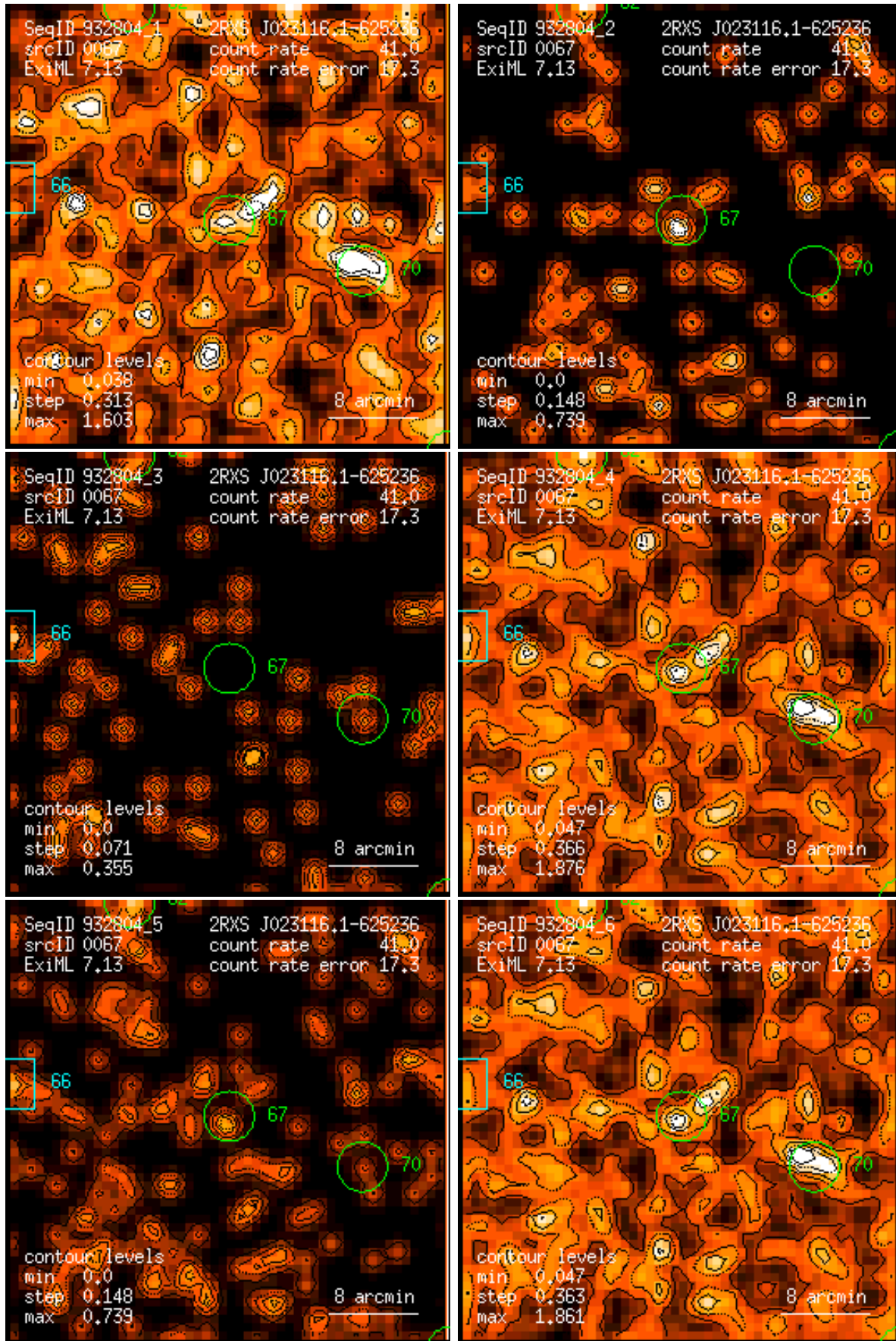
Figure 67: RASS 932804: detection 0067: band rate images, Gaussian filter: (1) PSPC channels 11 – 41, (2) 52 – 90, (3) 91 – 201, (4) 11 – 235, (5) 52 – 201, (6) 11 – 201. Broad band rates in counts/ks. Band rate contour levels in counts/ks/arcmin 2 .
