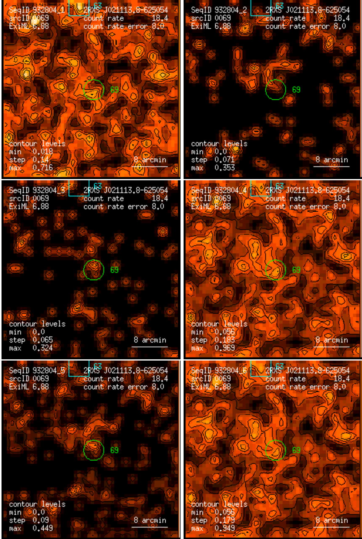
Figure 69: RASS 932804: detection 0069: band rate images, Gaussian filter: (1) PSPC channels 11 – 41, (2) 52 – 90, (3) 91 – 201, (4) 11 – 235, (5) 52 – 201, (6) 11 – 201. Broad band rates in counts/ks. Band rate contour levels in counts/ks/arcmin 2 .
