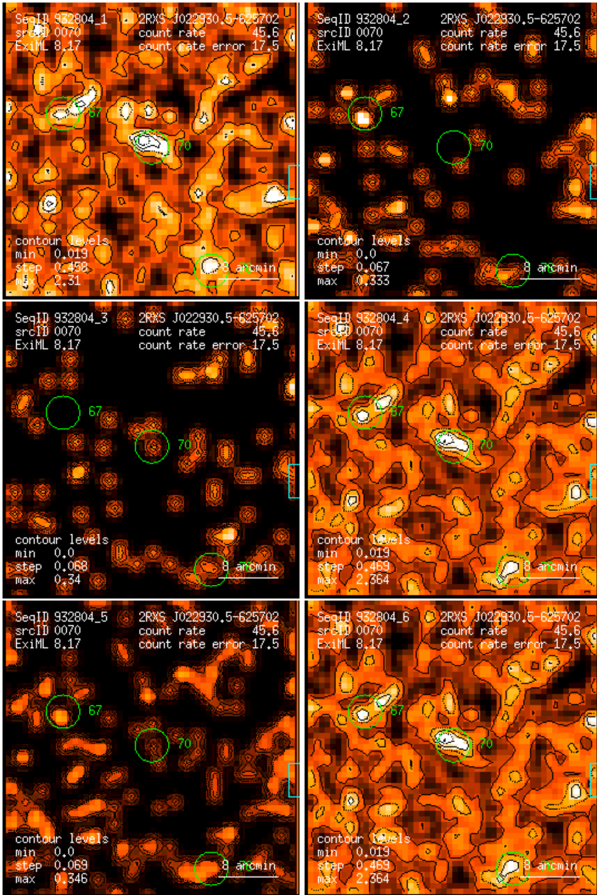
Figure 70: RASS 932804: detection 0070: band rate images, Gaussian filter: (1) PSPC channels 11 – 41, (2) 52 – 90, (3) 91 – 201, (4) 11 – 235, (5) 52 – 201, (6) 11 – 201. Broad band rates in counts/ks. Band rate contour levels in counts/ks/arcmin 2 .
