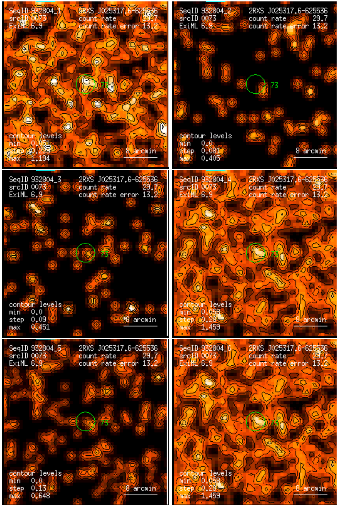
Figure 73: RASS 932804: detection 0073: band rate images, Gaussian filter: (1) PSPC channels 11 – 41, (2) 52 – 90, (3) 91 – 201, (4) 11 – 235, (5) 52 – 201, (6) 11 – 201. Broad band rates in counts/ks. Band rate contour levels in counts/ks/arcmin 2 .
