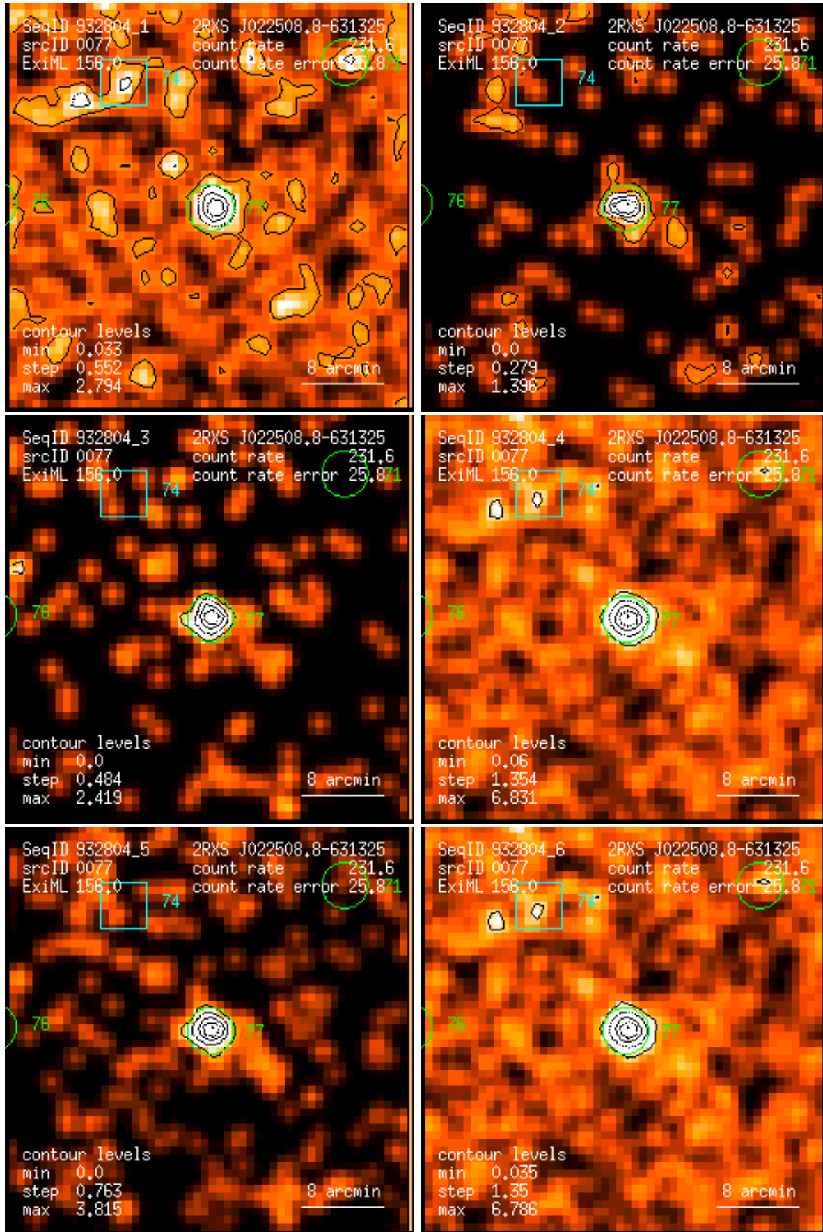
Figure 77: RASS 932804: detection 0077: band rate images, Gaussian filter: (1) PSPC channels 11 – 41, (2) 52 – 90, (3) 91 – 201, (4) 11 – 235, (5) 52 – 201, (6) 11 – 201. Broad band rates in counts/ks. Band rate contour levels in counts/ks/arcmin 2 .
