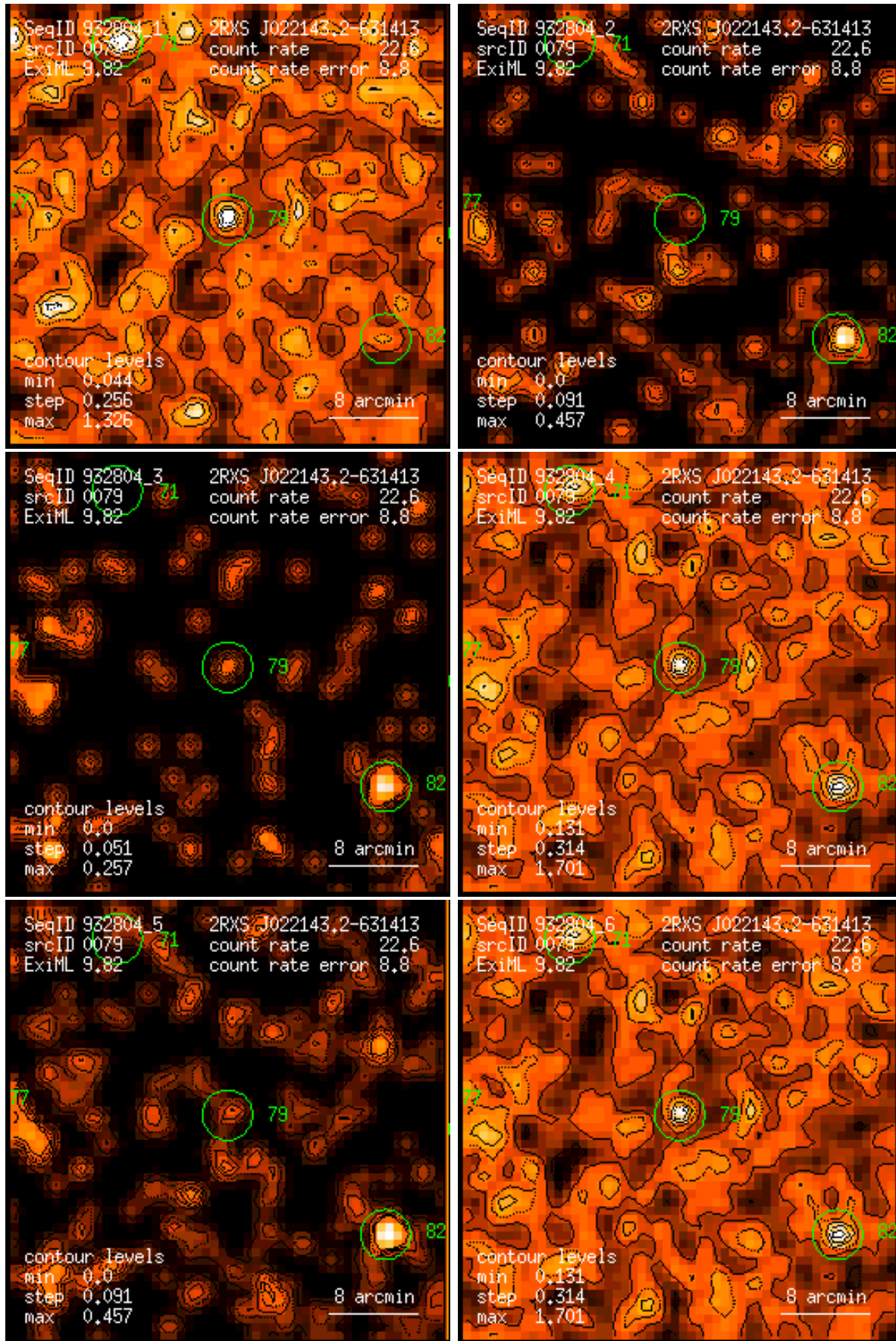
Figure 79: RASS 932804: detection 0079: band rate images, Gaussian filter: (1) PSPC channels 11 – 41, (2) 52 – 90, (3) 91 – 201, (4) 11 – 235, (5) 52 – 201, (6) 11 – 201. Broad band rates in counts/ks. Band rate contour levels in counts/ks/arcmin 2 .
