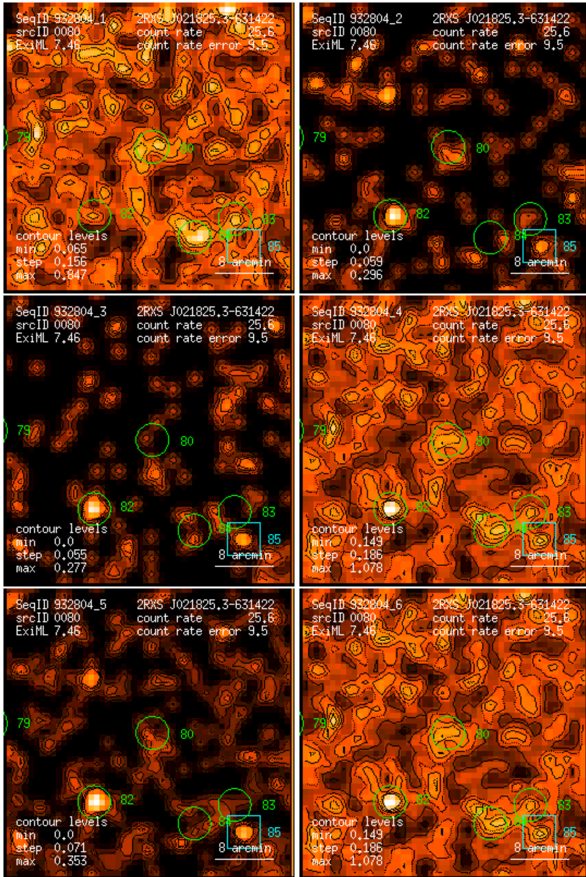
Figure 80: RASS 932804: detection 0080: band rate images, Gaussian filter: (1) PSPC channels 11 – 41, (2) 52 – 90, (3) 91 – 201, (4) 11 – 235, (5) 52 – 201, (6) 11 – 201. Broad band rates in counts/ks. Band rate contour levels in counts/ks/arcmin 2 .
