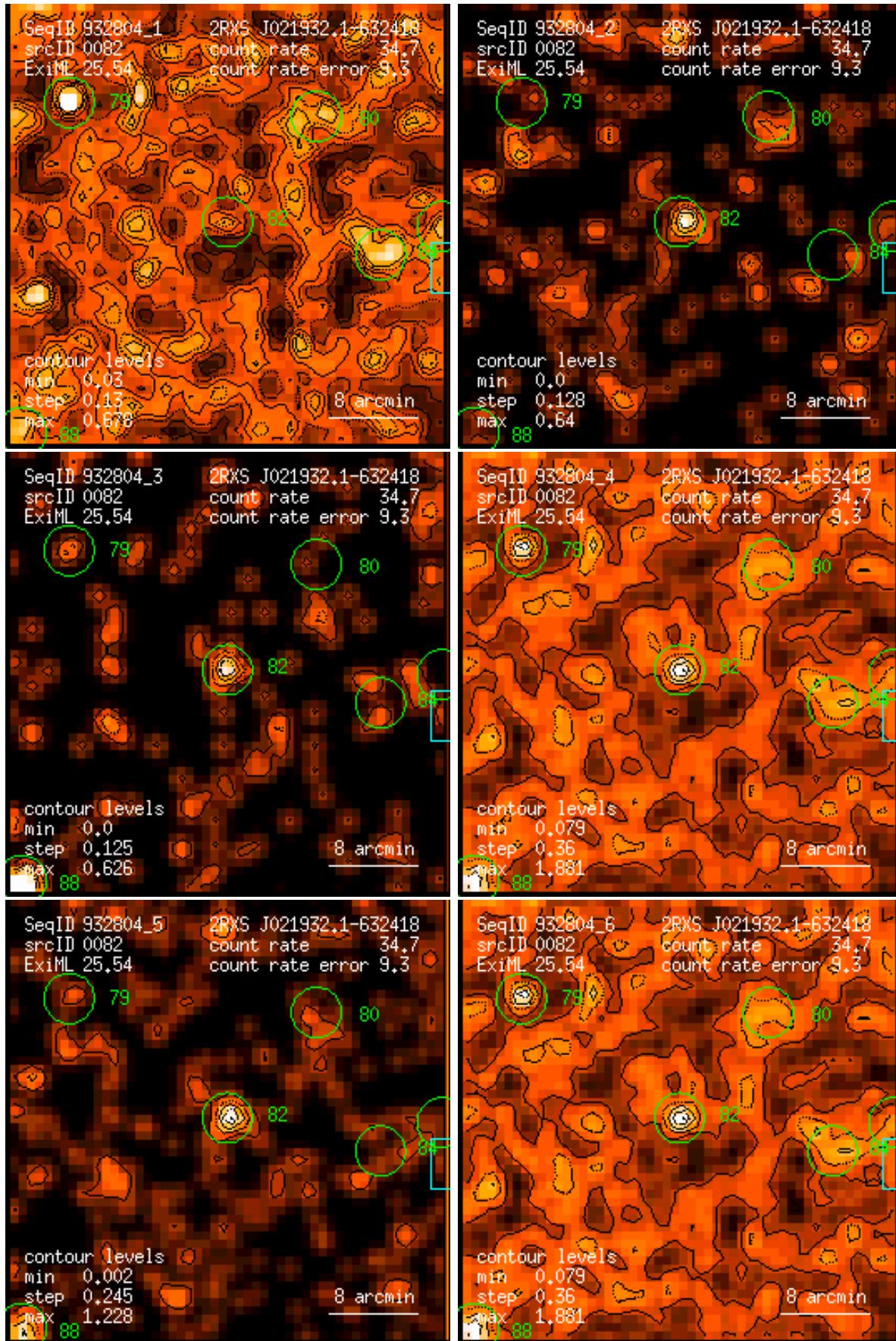
Figure 82: RASS 932804: detection 0082: band rate images, Gaussian filter: (1) PSPC channels 11 – 41, (2) 52 – 90, (3) 91 – 201, (4) 11 – 235, (5) 52 – 201, (6) 11 – 201. Broad band rates in counts/ks. Band rate contour levels in counts/ks/arcmin 2 .
