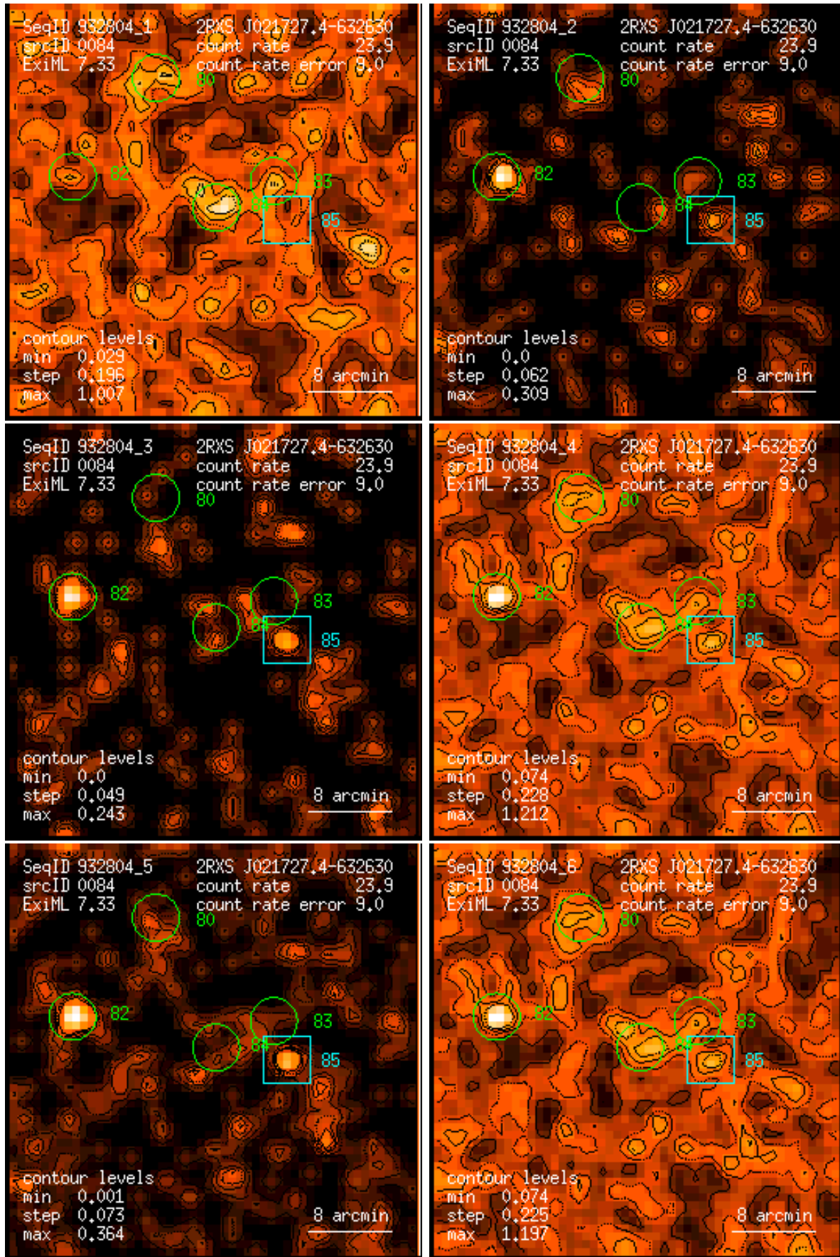
Figure 84: RASS 932804: detection 0084: band rate images, Gaussian filter: (1) PSPC channels 11 – 41, (2) 52 – 90, (3) 91 – 201, (4) 11 – 235, (5) 52 – 201, (6) 11 – 201. Broad band rates in counts/ks. Band rate contour levels in counts/ks/arcmin 2 .
