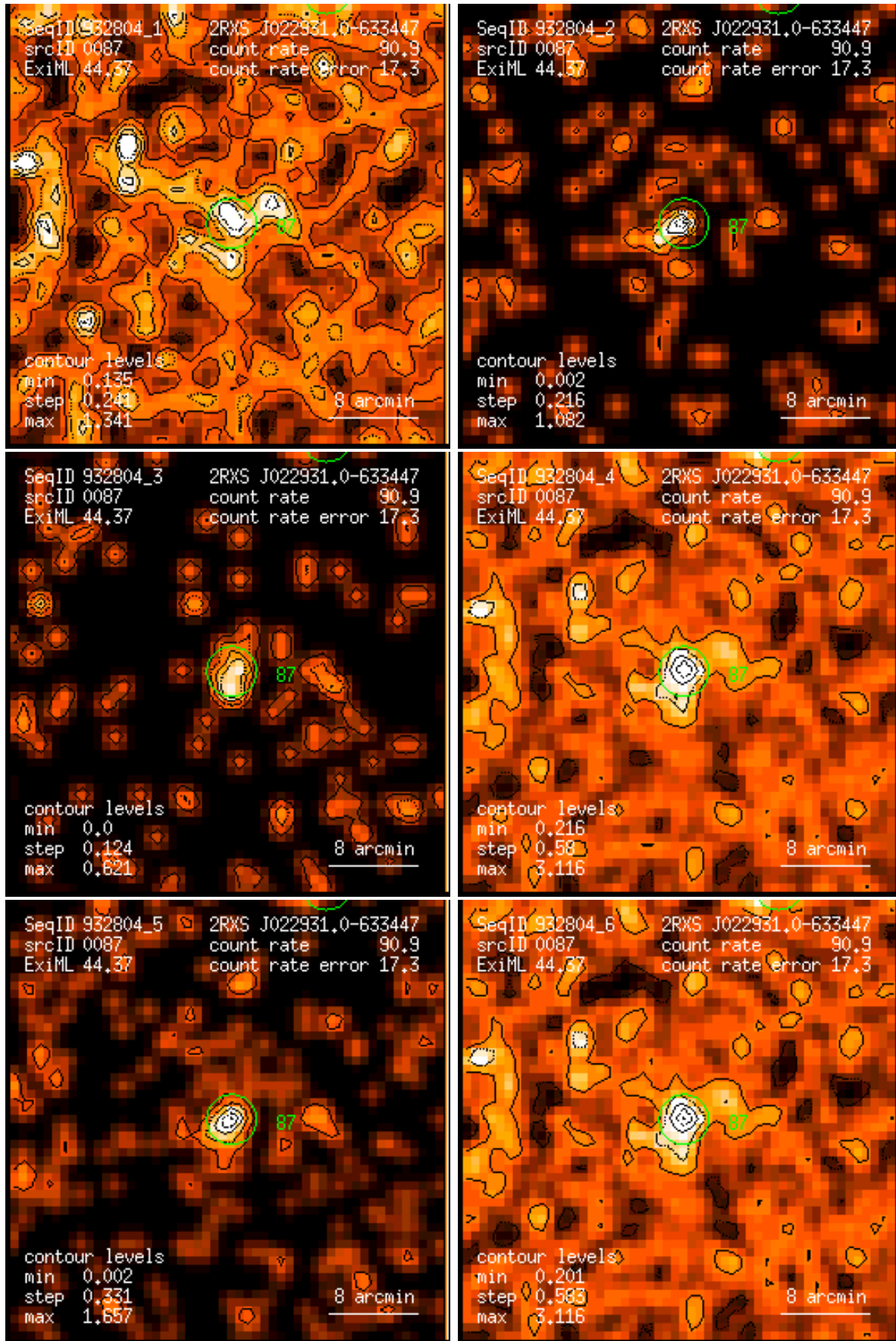
Figure 87: RASS 932804: detection 0087: band rate images, Gaussian filter: (1) PSPC channels 11 – 41, (2) 52 – 90, (3) 91 – 201, (4) 11 – 235, (5) 52 – 201, (6) 11 – 201. Broad band rates in counts/ks. Band rate contour levels in counts/ks/arcmin 2 .
