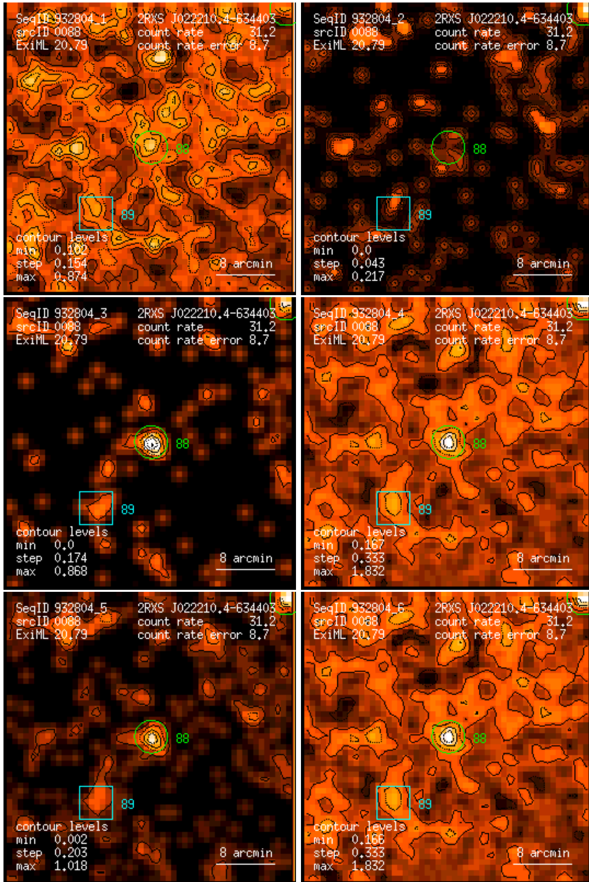
Figure 88: RASS 932804: detection 0088: band rate images, Gaussian filter: (1) PSPC channels 11 – 41, (2) 52 – 90, (3) 91 – 201, (4) 11 – 235, (5) 52 – 201, (6) 11 – 201. Broad band rates in counts/ks. Band rate contour levels in counts/ks/arcmin 2 .
