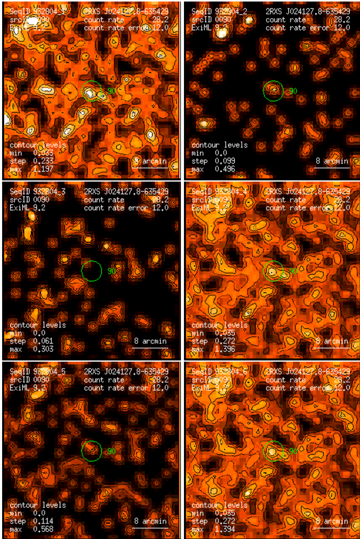
Figure 90: RASS 932804: detection 0090: band rate images, Gaussian filter: (1) PSPC channels 11 – 41, (2) 52 – 90, (3) 91 – 201, (4) 11 – 235, (5) 52 – 201, (6) 11 – 201. Broad band rates in counts/ks. Band rate contour levels in counts/ks/arcmin 2 .
