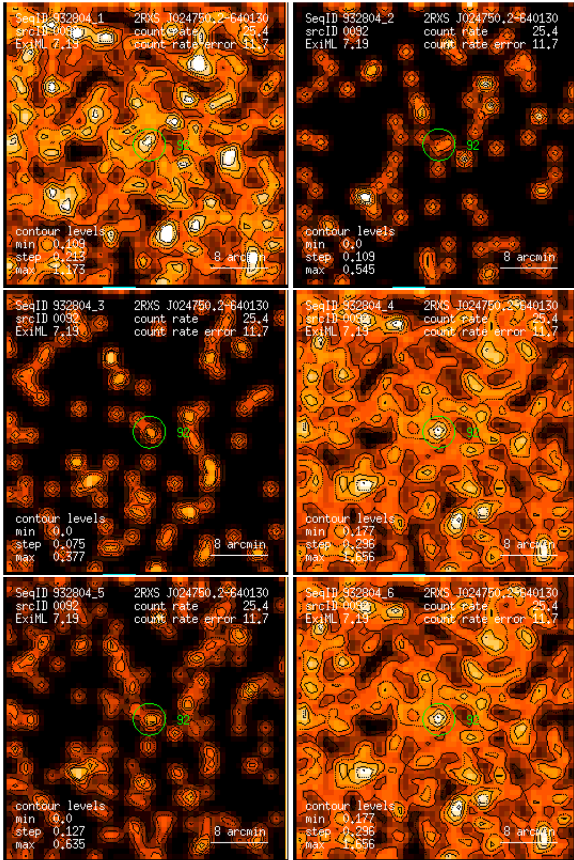
Figure 92: RASS 932804: detection 0092: band rate images, Gaussian filter: (1) PSPC channels 11 – 41, (2) 52 – 90, (3) 91 – 201, (4) 11 – 235, (5) 52 – 201, (6) 11 – 201. Broad band rates in counts/ks. Band rate contour levels in counts/ks/arcmin 2 .
