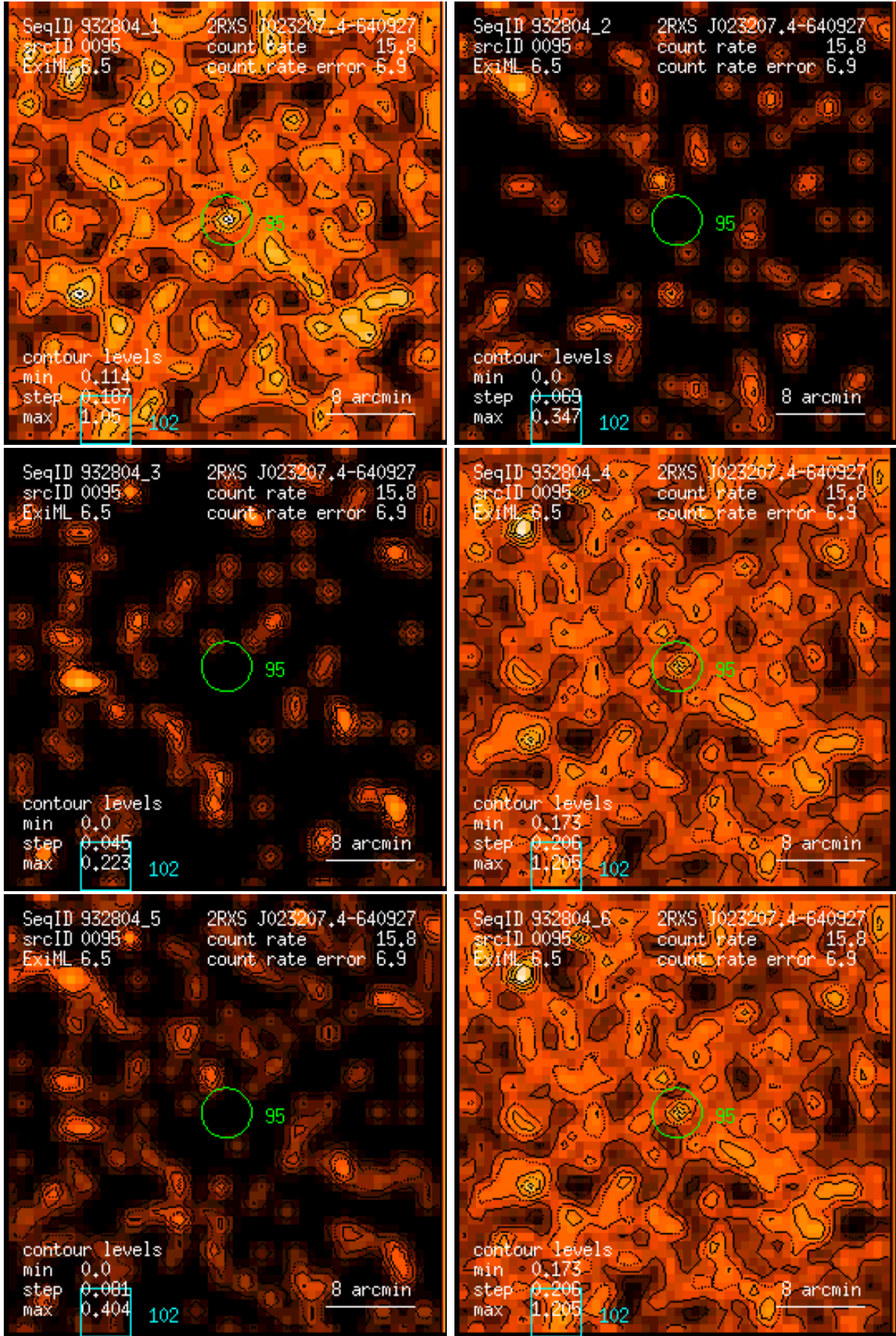
Figure 95: RASS 932804: detection 0095: band rate images, Gaussian filter: (1) PSPC channels 11 – 41, (2) 52 – 90, (3) 91 – 201, (4) 11 – 235, (5) 52 – 201, (6) 11 – 201. Broad band rates in counts/ks. Band rate contour levels in counts/ks/arcmin 2 .
