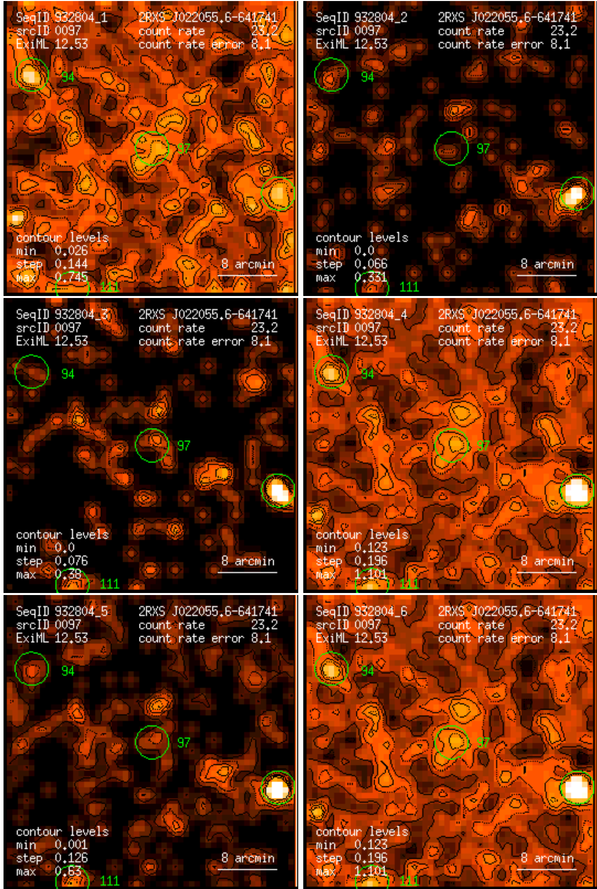
Figure 97: RASS 932804: detection 0097: band rate images, Gaussian filter: (1) PSPC channels 11 – 41, (2) 52 – 90, (3) 91 – 201, (4) 11 – 235, (5) 52 – 201, (6) 11 – 201. Broad band rates in counts/ks. Band rate contour levels in counts/ks/arcmin 2 .
