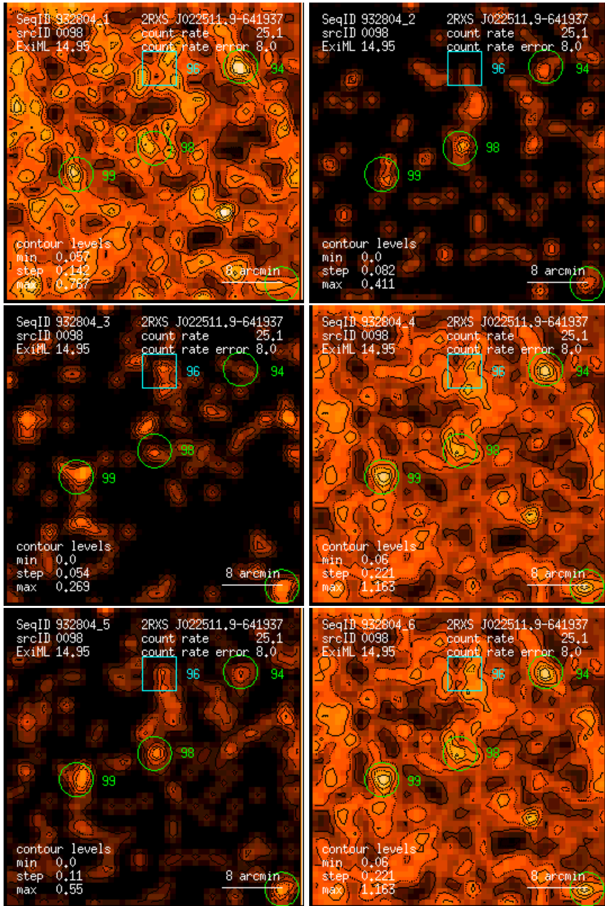
Figure 98: RASS 932804: detection 0098: band rate images, Gaussian filter: (1) PSPC channels 11 – 41, (2) 52 – 90, (3) 91 – 201, (4) 11 – 235, (5) 52 – 201, (6) 11 – 201. Broad band rates in counts/ks. Band rate contour levels in counts/ks/arcmin 2 .
