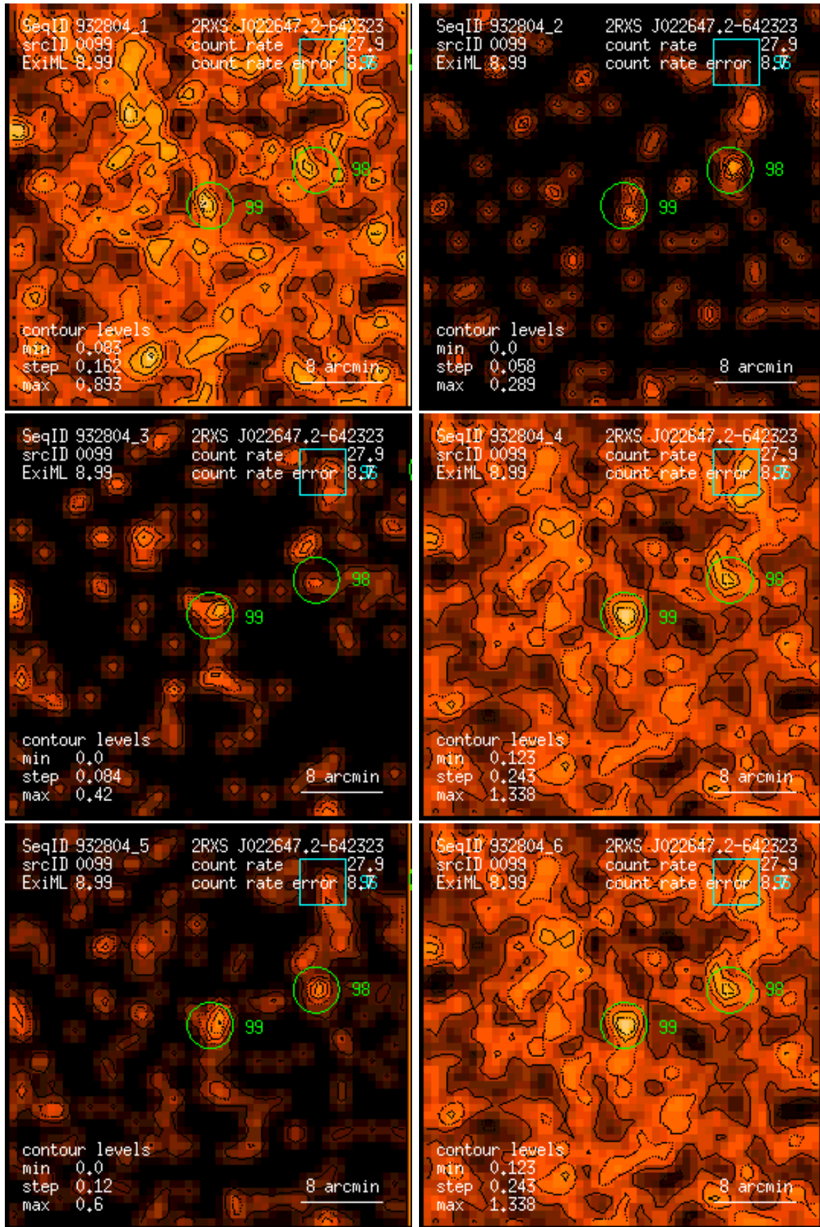
Figure 99: RASS 932804: detection 0099: band rate images, Gaussian filter: (1) PSPC channels 11 – 41, (2) 52 – 90, (3) 91 – 201, (4) 11 – 235, (5) 52 – 201, (6) 11 – 201. Broad band rates in counts/ks. Band rate contour levels in counts/ks/arcmin 2 .
