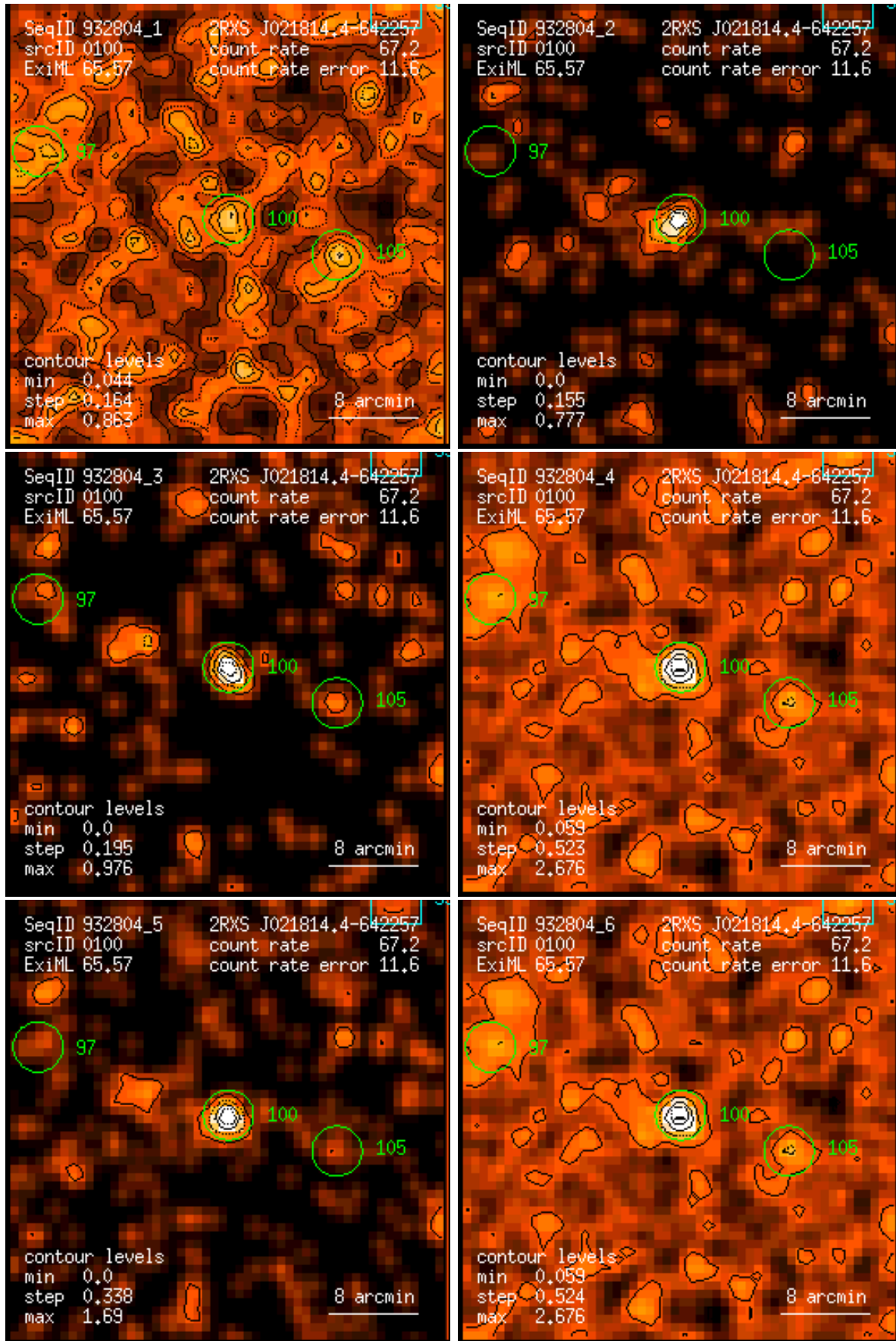
Figure 100: RASS 932804: detection 0100: band rate images, Gaussian filter: (1) PSPC channels 11 – 41, (2) 52 – 90, (3) 91 – 201, (4) 11 – 235, (5) 52 – 201, (6) 11 – 201. Broad band rates in counts/ks. Band rate contour levels in counts/ks/arcmin 2 .
