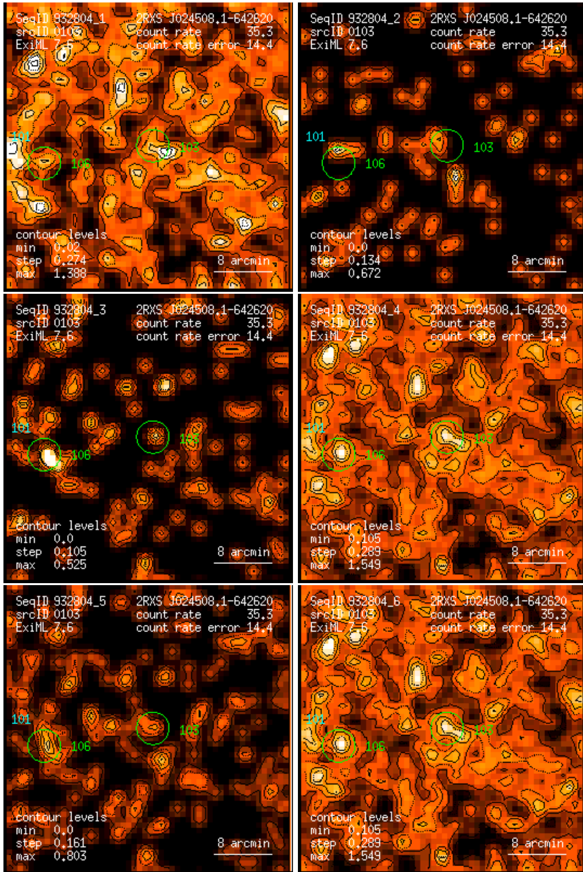
Figure 103: RASS 932804: detection 0103: band rate images, Gaussian filter: (1) PSPC channels 11 – 41, (2) 52 – 90, (3) 91 – 201, (4) 11 – 235, (5) 52 – 201, (6) 11 – 201. Broad band rates in counts/ks. Band rate contour levels in counts/ks/arcmin 2 .
