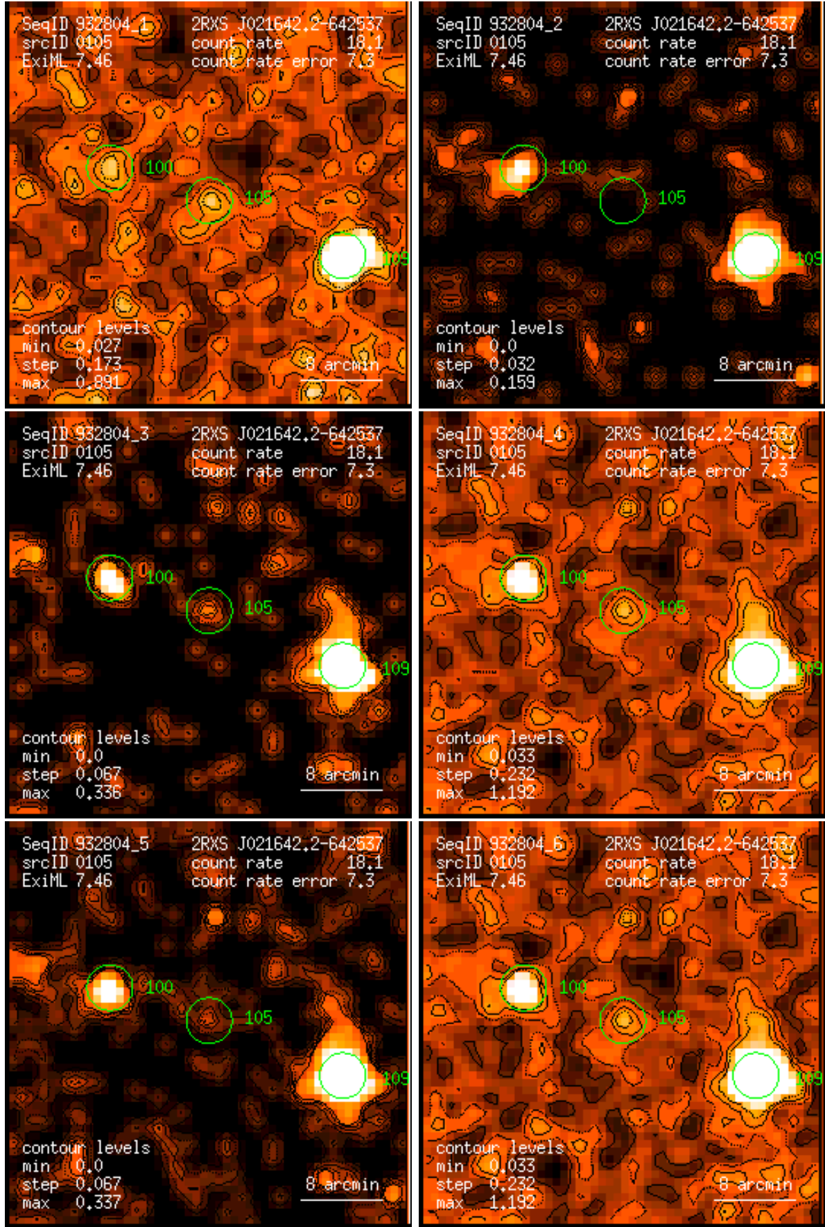
Figure 105: RASS 932804: detection 0105: band rate images, Gaussian filter: (1) PSPC channels 11 – 41, (2) 52 – 90, (3) 91 – 201, (4) 11 – 235, (5) 52 – 201, (6) 11 – 201. Broad band rates in counts/ks. Band rate contour levels in counts/ks/arcmin 2 .
