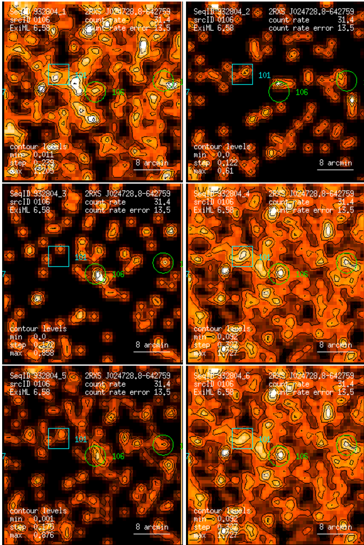
Figure 106: RASS 932804: detection 0106: band rate images, Gaussian filter: (1) PSPC channels 11 – 41, (2) 52 – 90, (3) 91 – 201, (4) 11 – 235, (5) 52 – 201, (6) 11 – 201. Broad band rates in counts/ks. Band rate contour levels in counts/ks/arcmin 2 .
