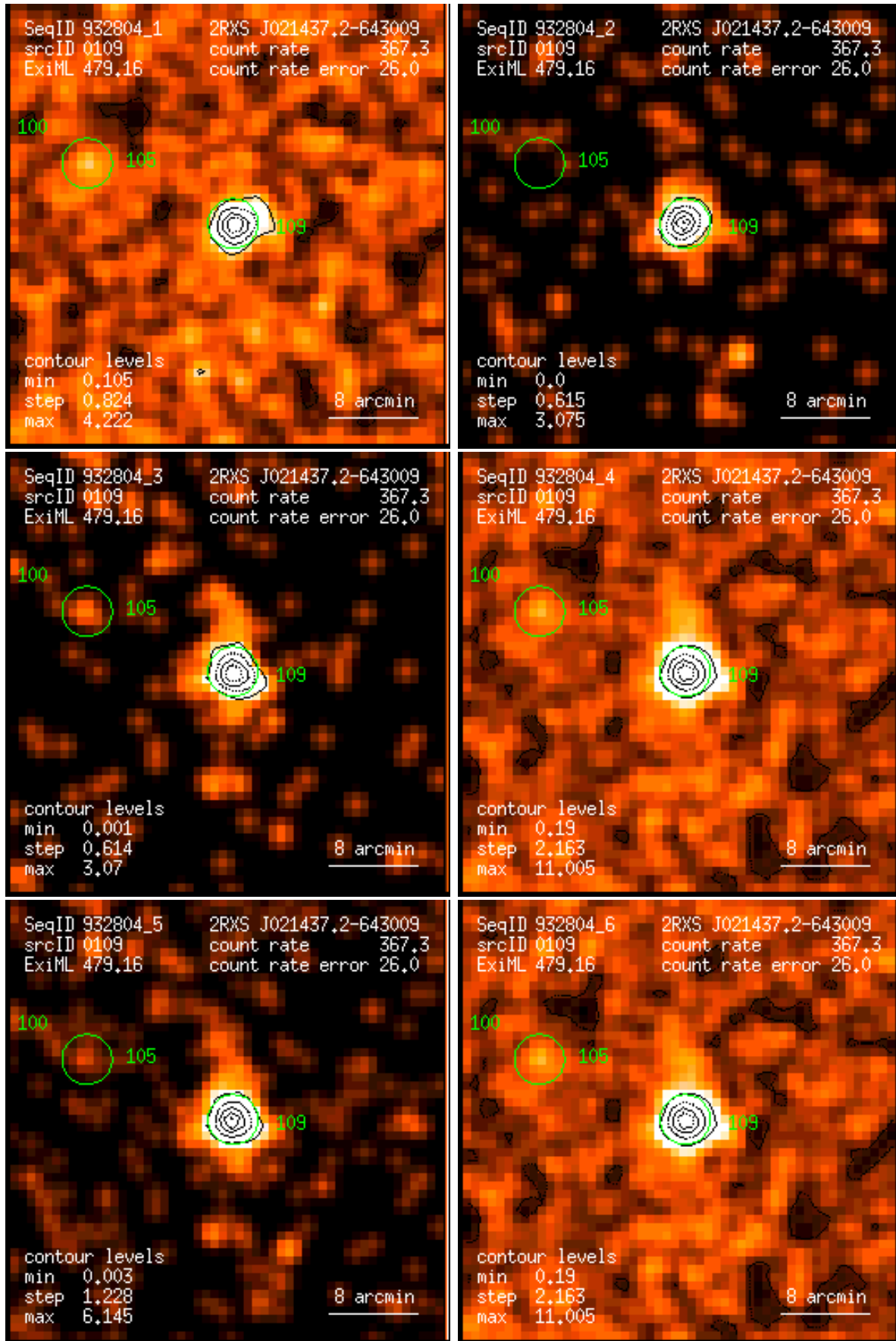
Figure 109: RASS 932804: detection 0109: band rate images, Gaussian filter: (1) PSPC channels 11 – 41, (2) 52 – 90, (3) 91 – 201, (4) 11 – 235, (5) 52 – 201, (6) 11 – 201. Broad band rates in counts/ks. Band rate contour levels in counts/ks/arcmin 2 .
