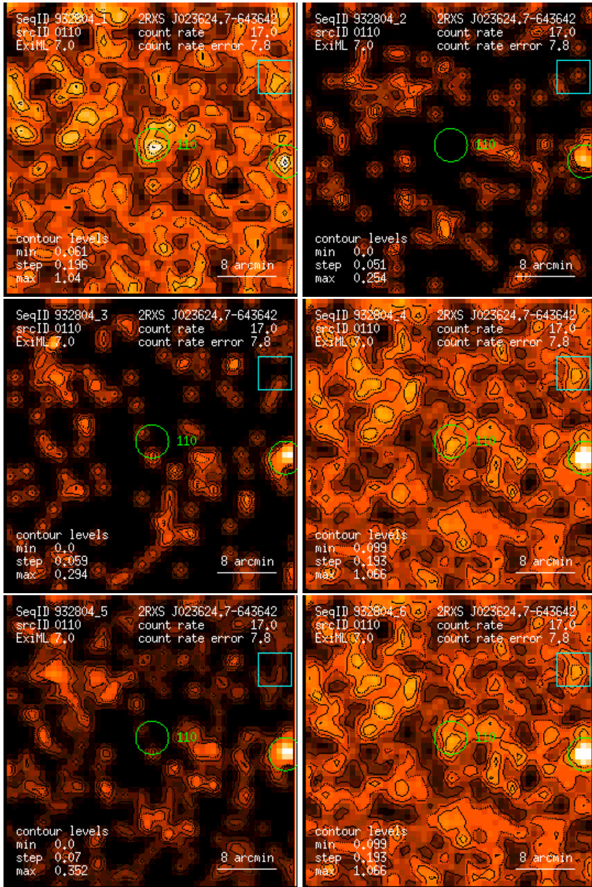
Figure 110: RASS 932804: detection 0110: band rate images, Gaussian filter: (1) PSPC channels 11 – 41, (2) 52 – 90, (3) 91 – 201, (4) 11 – 235, (5) 52 – 201, (6) 11 – 201. Broad band rates in counts/ks. Band rate contour levels in counts/ks/arcmin 2 .
