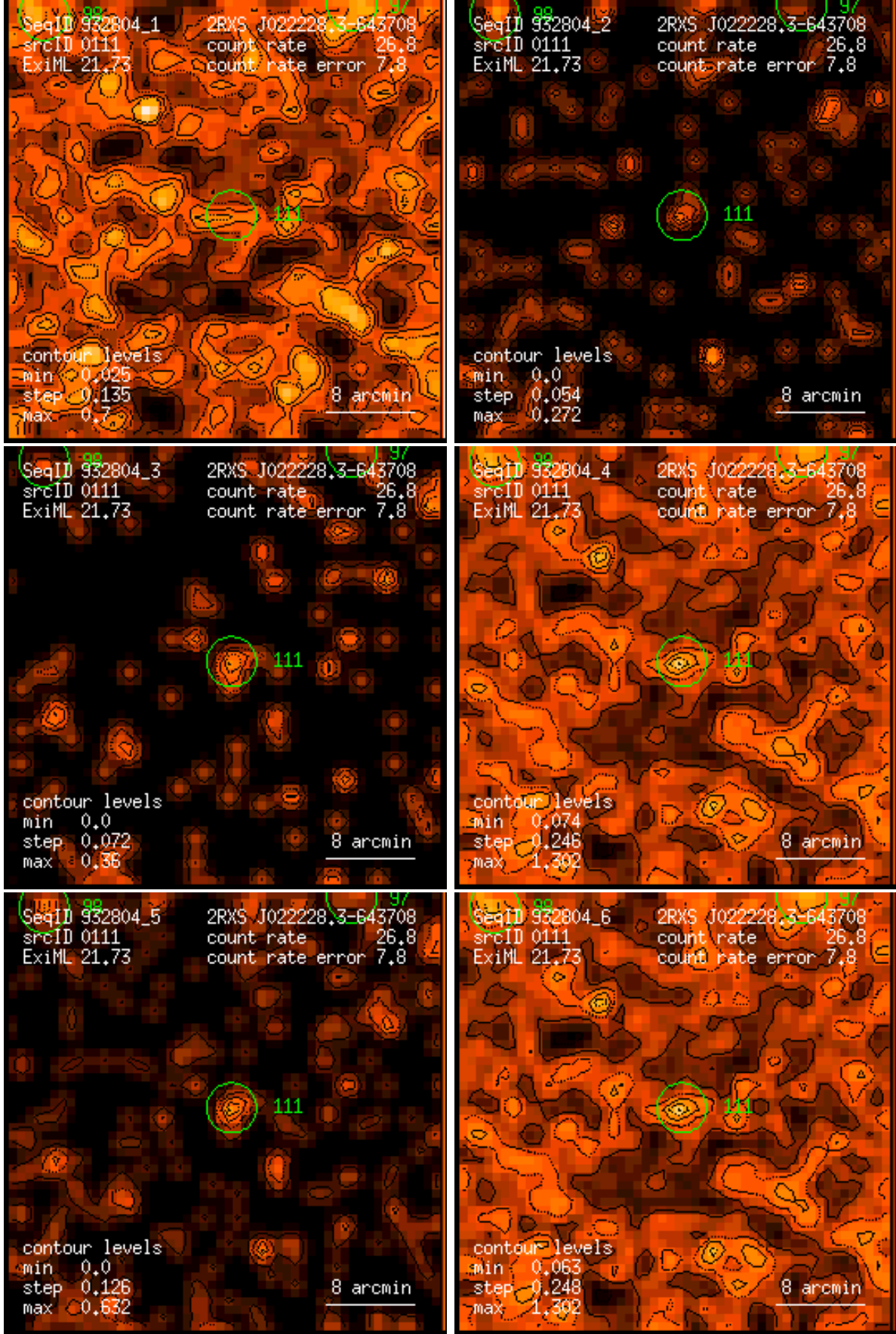
Figure 111: RASS 932804: detection 0111: band rate images, Gaussian filter: (1) PSPC channels 11 – 41, (2) 52 – 90, (3) 91 – 201, (4) 11 – 235, (5) 52 – 201, (6) 11 – 201. Broad band rates in counts/ks. Band rate contour levels in counts/ks/arcmin 2 .
