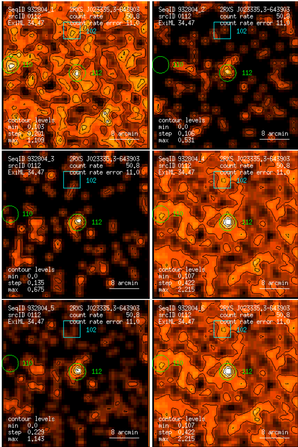
Figure 112: RASS 932804: detection 0112: band rate images, Gaussian filter: (1) PSPC channels 11 – 41, (2) 52 – 90, (3) 91 – 201, (4) 11 – 235, (5) 52 – 201, (6) 11 – 201. Broad band rates in counts/ks. Band rate contour levels in counts/ks/arcmin 2 .
