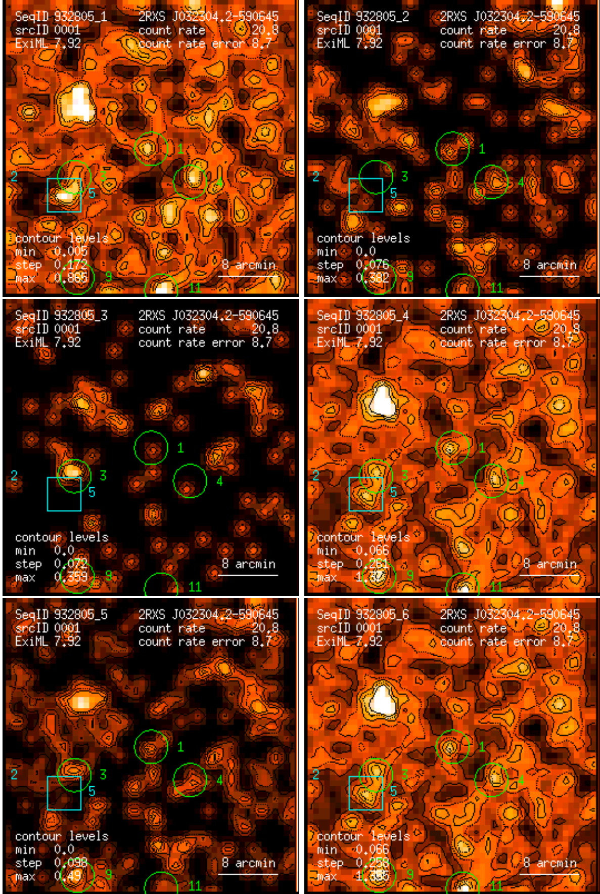
Figure 1: RASS 932805: detection 0001: band rate images, Gaussian filter: (1) PSPC channels 11 – 41, (2) 52 – 90, (3) 91 – 201, (4) 11 – 235, (5) 52 – 201, (6) 11 – 201. Broad band rates in counts/ks. Band rate contour levels in counts/ks/arcmin 2 .
