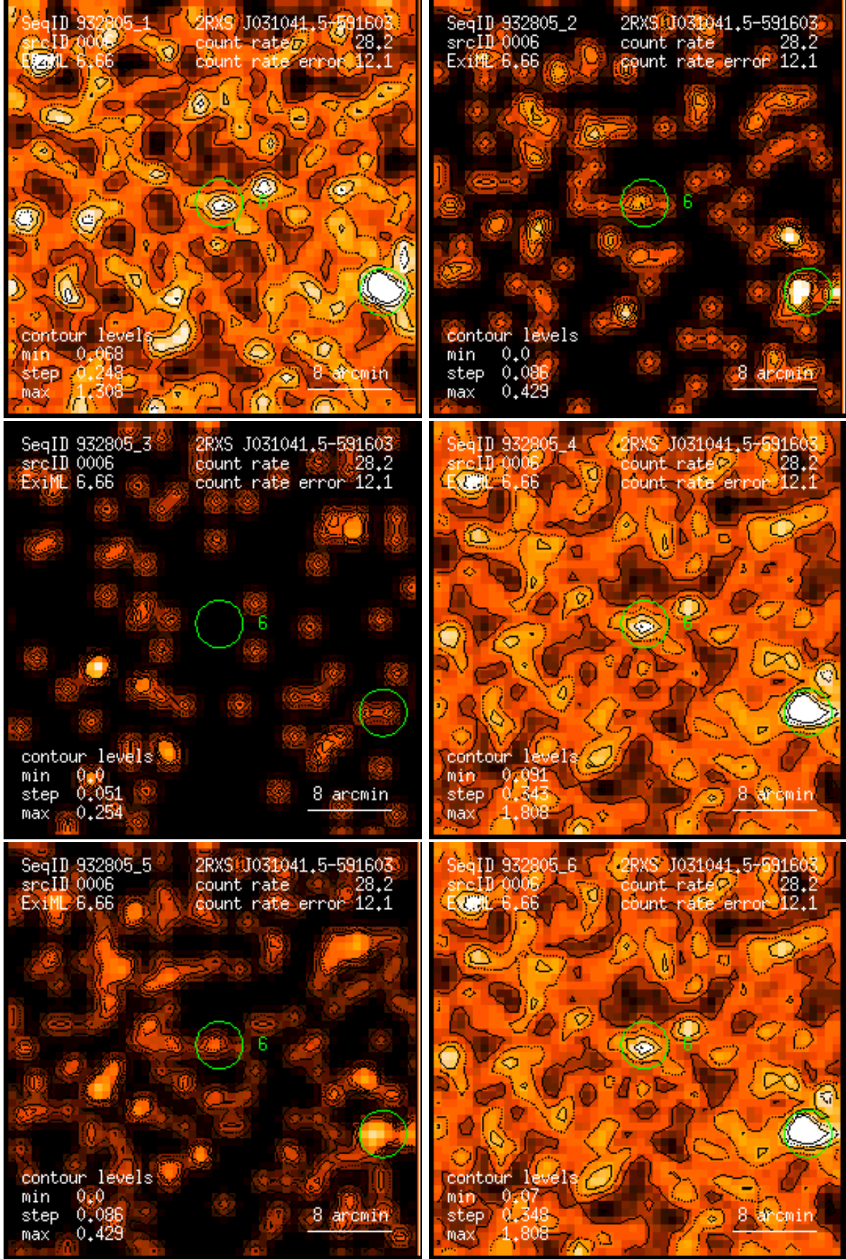
Figure 6: RASS 932805: detection 0006: band rate images, Gaussian filter: (1) PSPC channels 11 – 41, (2) 52 – 90, (3) 91 – 201, (4) 11 – 235, (5) 52 – 201, (6) 11 – 201. Broad band rates in counts/ks. Band rate contour levels in counts/ks/arcmin 2 .
