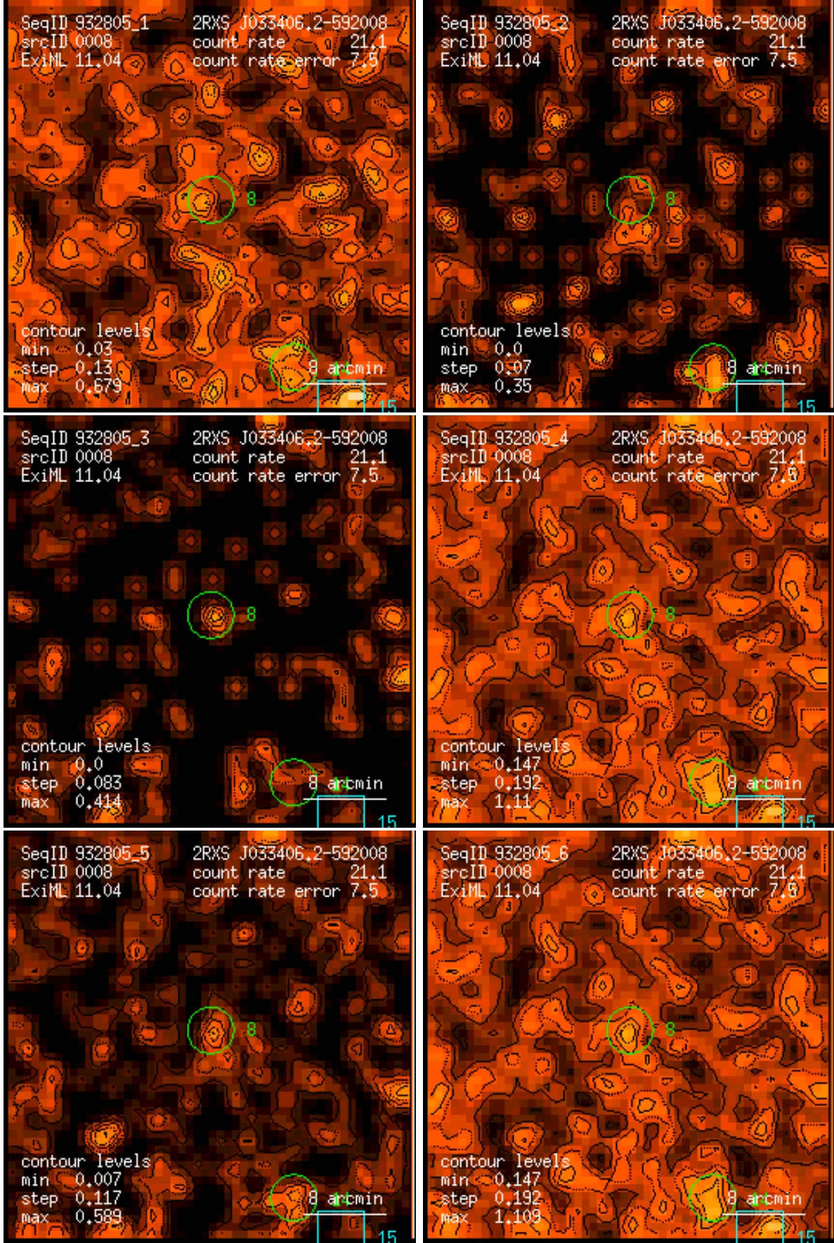
Figure 8: RASS 932805: detection 0008: band rate images, Gaussian filter: (1) PSPC channels 11 – 41, (2) 52 – 90, (3) 91 – 201, (4) 11 – 235, (5) 52 – 201, (6) 11 – 201. Broad band rates in counts/ks. Band rate contour levels in counts/ks/arcmin 2 .
