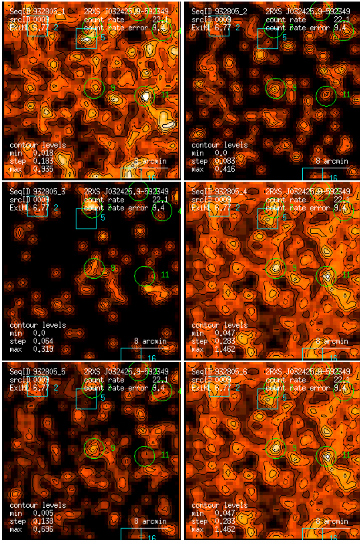
Figure 9: RASS 932805: detection 0009: band rate images, Gaussian filter: (1) PSPC channels 11 – 41, (2) 52 – 90, (3) 91 – 201, (4) 11 – 235, (5) 52 – 201, (6) 11 – 201. Broad band rates in counts/ks. Band rate contour levels in counts/ks/arcmin 2 .
