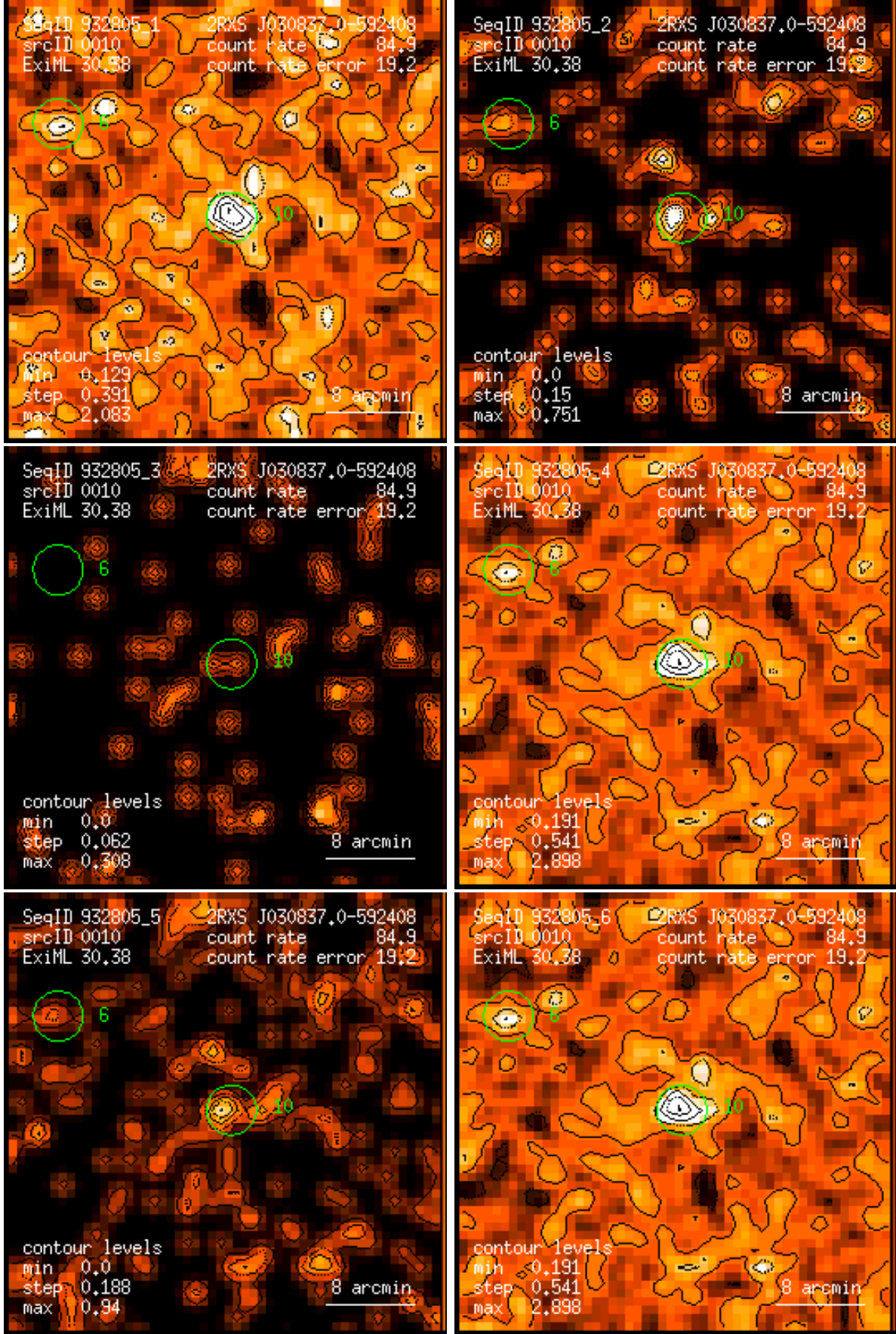
Figure 10: RASS 932805: detection 0010: band rate images, Gaussian filter: (1) PSPC channels 11 – 41, (2) 52 – 90, (3) 91 – 201, (4) 11 – 235, (5) 52 – 201, (6) 11 – 201. Broad band rates in counts/ks. Band rate contour levels in counts/ks/arcmin 2 .
