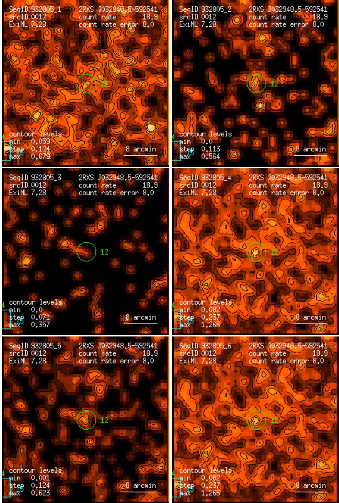
Figure 12: RASS 932805: detection 0012: band rate images, Gaussian filter: (1) PSPC channels 11 – 41, (2) 52 – 90, (3) 91 – 201, (4) 11 – 235, (5) 52 – 201, (6) 11 – 201. Broad band rates in counts/ks. Band rate contour levels in counts/ks/arcmin 2 .
