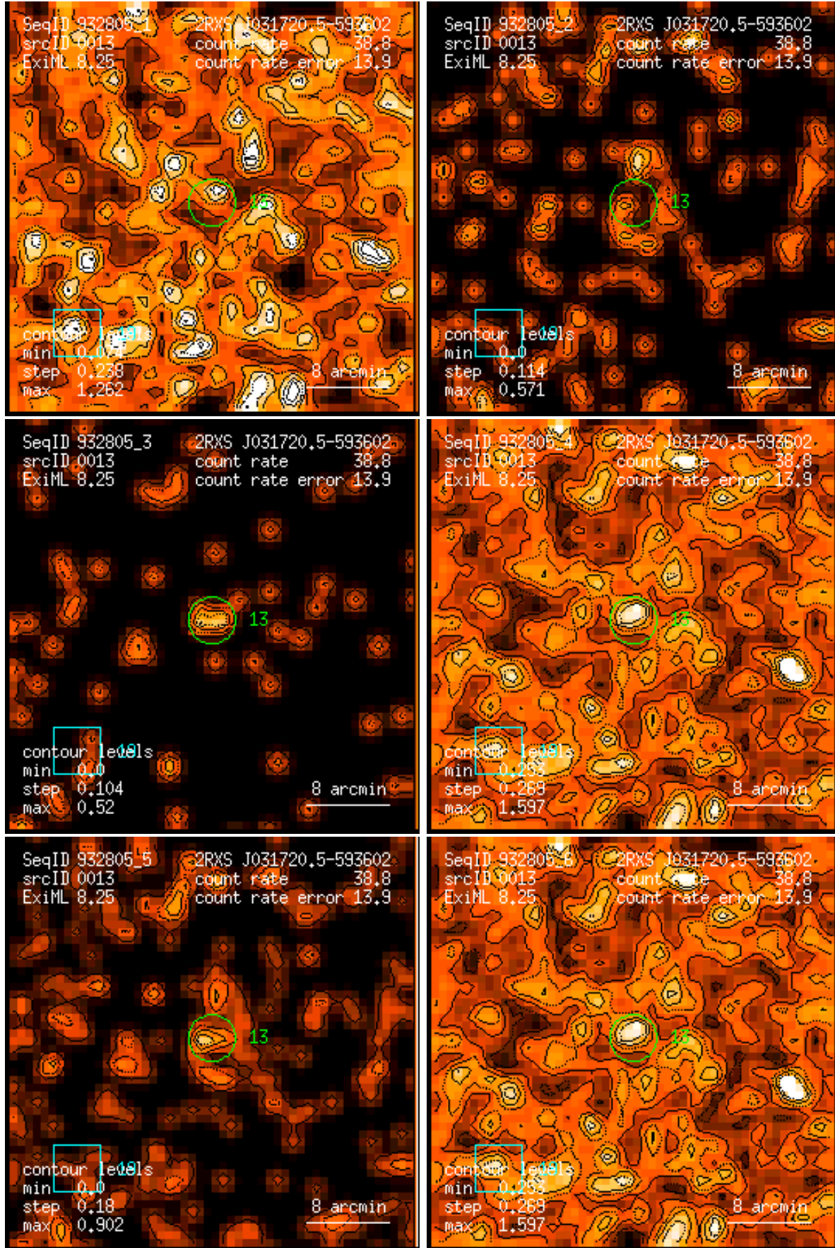
Figure 13: RASS 932805: detection 0013: band rate images, Gaussian filter: (1) PSPC channels 11 – 41, (2) 52 – 90, (3) 91 – 201, (4) 11 – 235, (5) 52 – 201, (6) 11 – 201. Broad band rates in counts/ks. Band rate contour levels in counts/ks/arcmin 2 .
