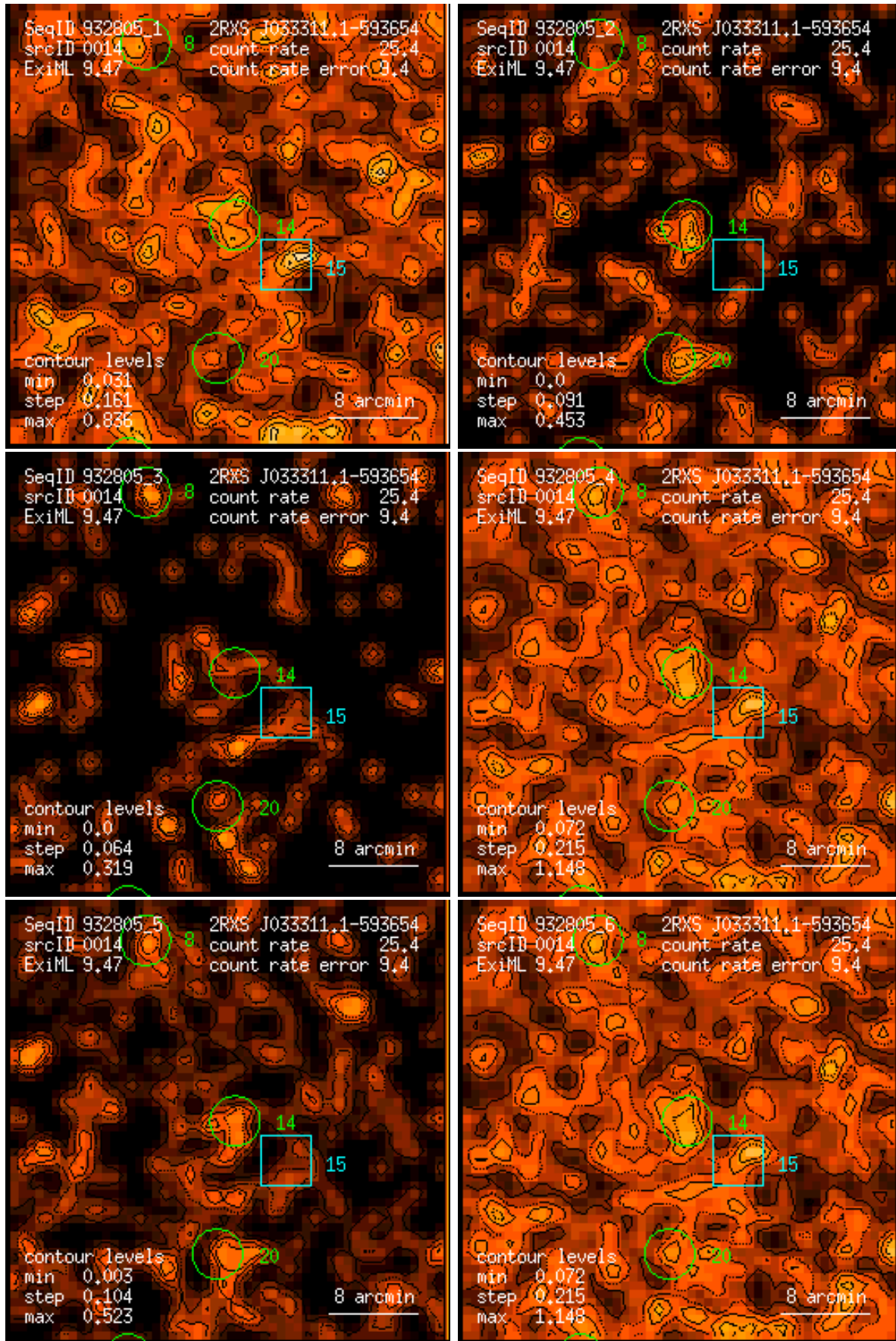
Figure 14: RASS 932805: detection 0014: band rate images, Gaussian filter: (1) PSPC channels 11 – 41, (2) 52 – 90, (3) 91 – 201, (4) 11 – 235, (5) 52 – 201, (6) 11 – 201. Broad band rates in counts/ks. Band rate contour levels in counts/ks/arcmin 2 .
