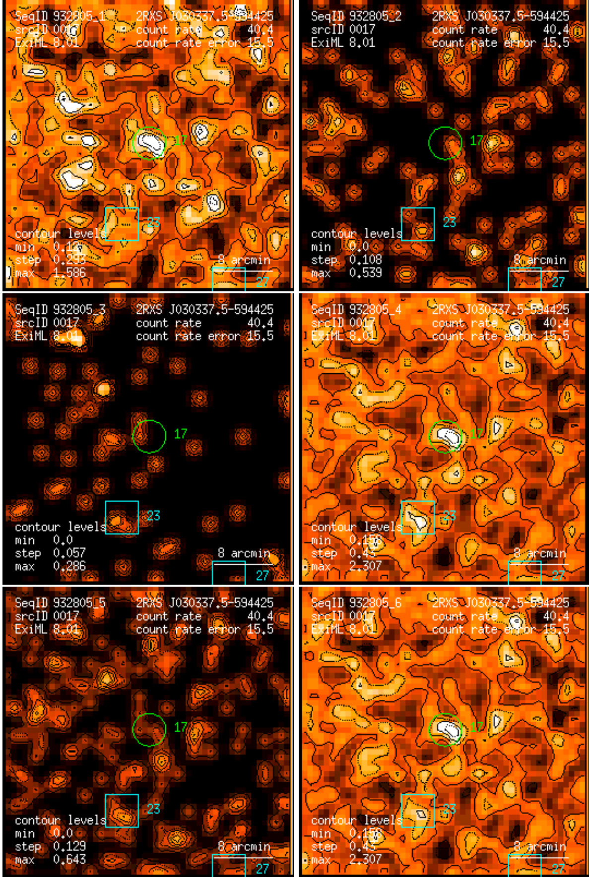
Figure 17: RASS 932805: detection 0017: band rate images, Gaussian filter: (1) PSPC channels 11 – 41, (2) 52 – 90, (3) 91 – 201, (4) 11 – 235, (5) 52 – 201, (6) 11 – 201. Broad band rates in counts/ks. Band rate contour levels in counts/ks/arcmin 2 .
