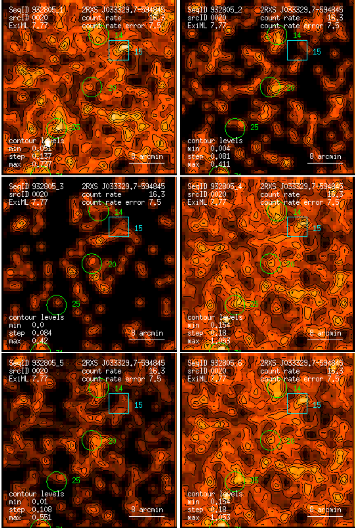
Figure 20: RASS 932805: detection 0020: band rate images, Gaussian filter: (1) PSPC channels 11 – 41, (2) 52 – 90, (3) 91 – 201, (4) 11 – 235, (5) 52 – 201, (6) 11 – 201. Broad band rates in counts/ks. Band rate contour levels in counts/ks/arcmin 2 .
