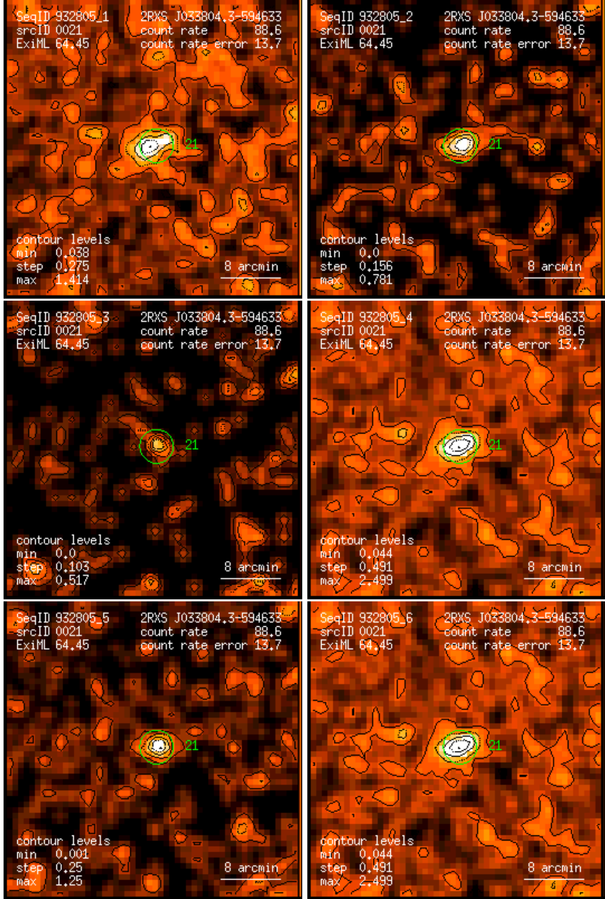
Figure 21: RASS 932805: detection 0021: band rate images, Gaussian filter: (1) PSPC channels 11 – 41, (2) 52 – 90, (3) 91 – 201, (4) 11 – 235, (5) 52 – 201, (6) 11 – 201. Broad band rates in counts/ks. Band rate contour levels in counts/ks/arcmin 2 .
