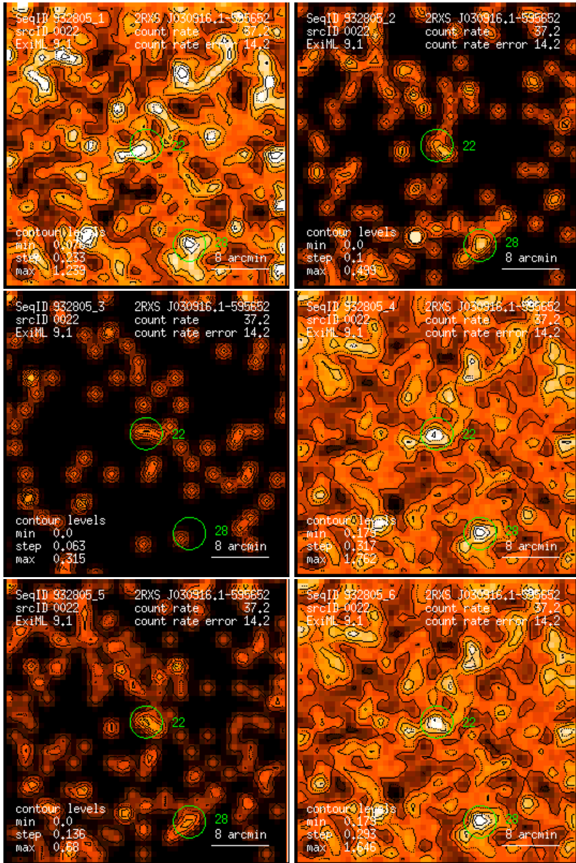
Figure 22: RASS 932805: detection 0022: band rate images, Gaussian filter: (1) PSPC channels 11 – 41, (2) 52 – 90, (3) 91 – 201, (4) 11 – 235, (5) 52 – 201, (6) 11 – 201. Broad band rates in counts/ks. Band rate contour levels in counts/ks/arcmin 2 .
