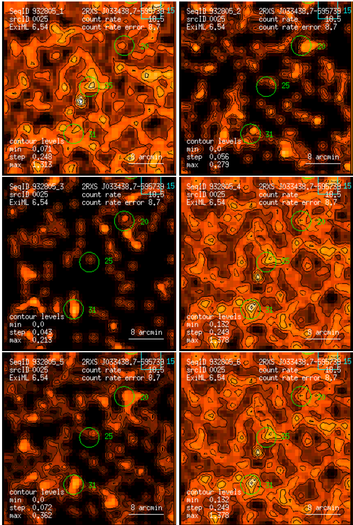
Figure 25: RASS 932805: detection 0025: band rate images, Gaussian filter: (1) PSPC channels 11 – 41, (2) 52 – 90, (3) 91 – 201, (4) 11 – 235, (5) 52 – 201, (6) 11 – 201. Broad band rates in counts/ks. Band rate contour levels in counts/ks/arcmin 2 .
