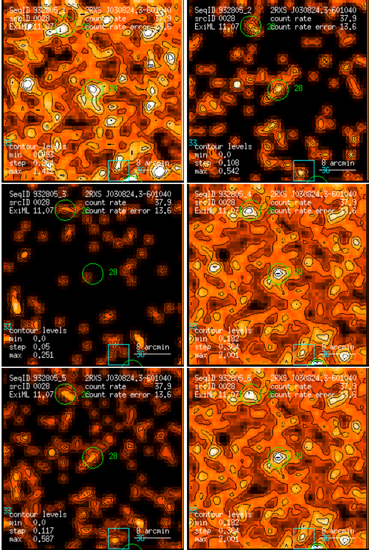
Figure 28: RASS 932805: detection 0028: band rate images, Gaussian filter: (1) PSPC channels 11 – 41, (2) 52 – 90, (3) 91 – 201, (4) 11 – 235, (5) 52 – 201, (6) 11 – 201. Broad band rates in counts/ks. Band rate contour levels in counts/ks/arcmin 2 .
