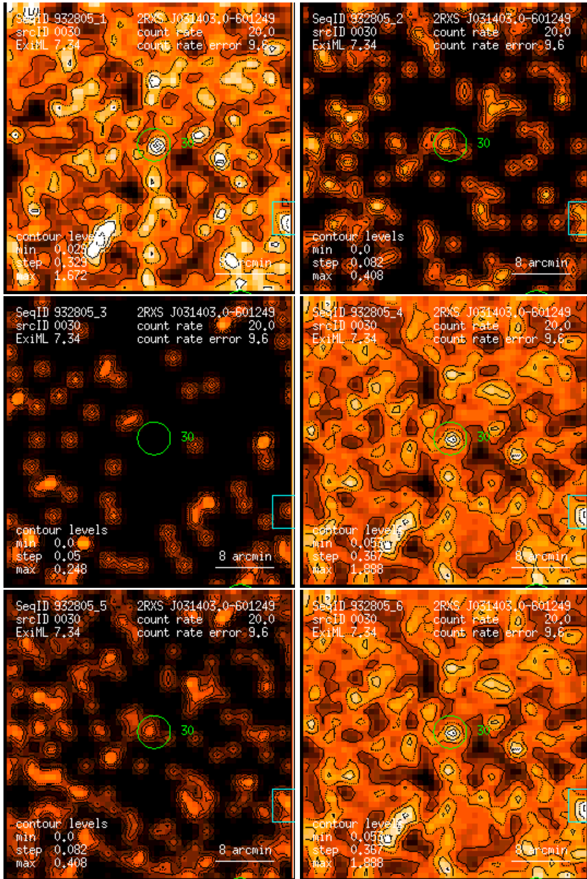
Figure 30: RASS 932805: detection 0030: band rate images, Gaussian filter: (1) PSPC channels 11 – 41, (2) 52 – 90, (3) 91 – 201, (4) 11 – 235, (5) 52 – 201, (6) 11 – 201. Broad band rates in counts/ks. Band rate contour levels in counts/ks/arcmin 2 .
