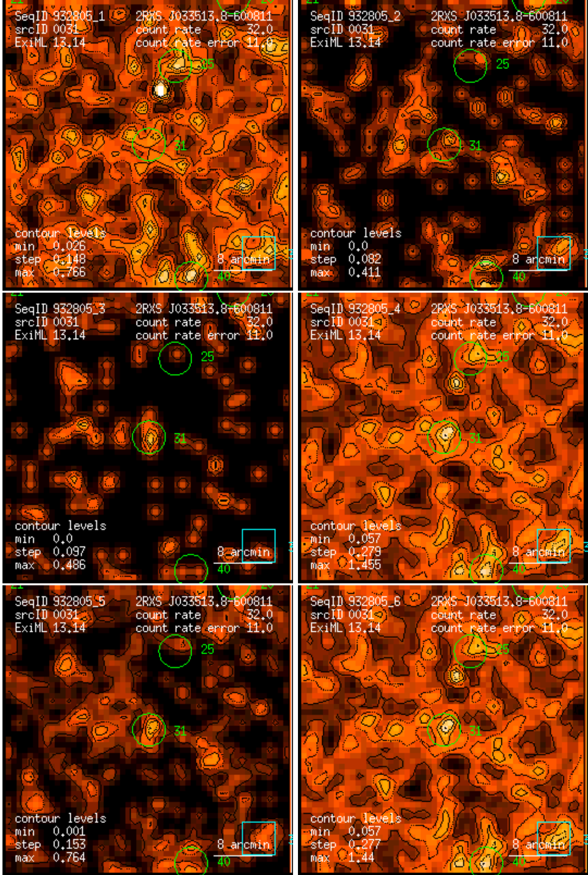
Figure 31: RASS 932805: detection 0031: band rate images, Gaussian filter: (1) PSPC channels 11 – 41, (2) 52 – 90, (3) 91 – 201, (4) 11 – 235, (5) 52 – 201, (6) 11 – 201. Broad band rates in counts/ks. Band rate contour levels in counts/ks/arcmin 2 .
