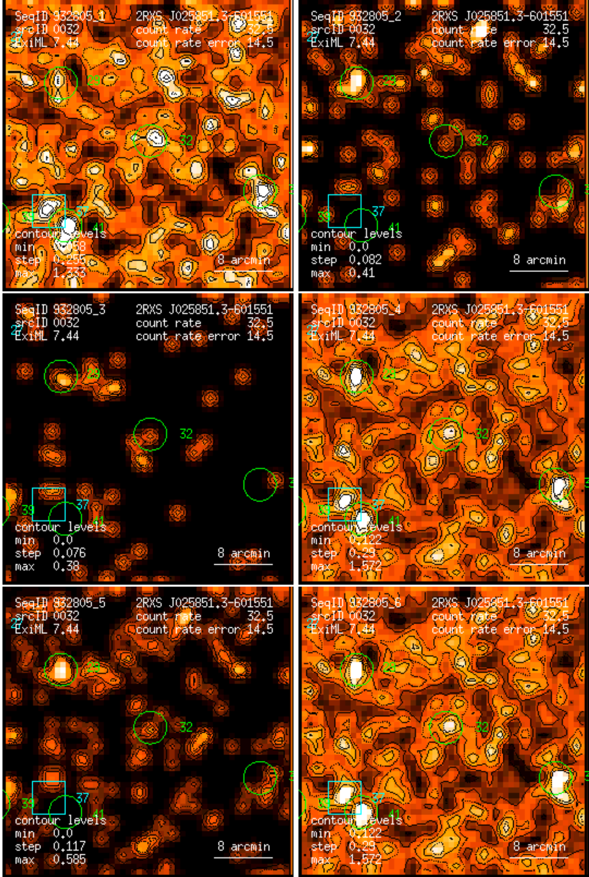
Figure 32: RASS 932805: detection 0032: band rate images, Gaussian filter: (1) PSPC channels 11 – 41, (2) 52 – 90, (3) 91 – 201, (4) 11 – 235, (5) 52 – 201, (6) 11 – 201. Broad band rates in counts/ks. Band rate contour levels in counts/ks/arcmin 2 .
