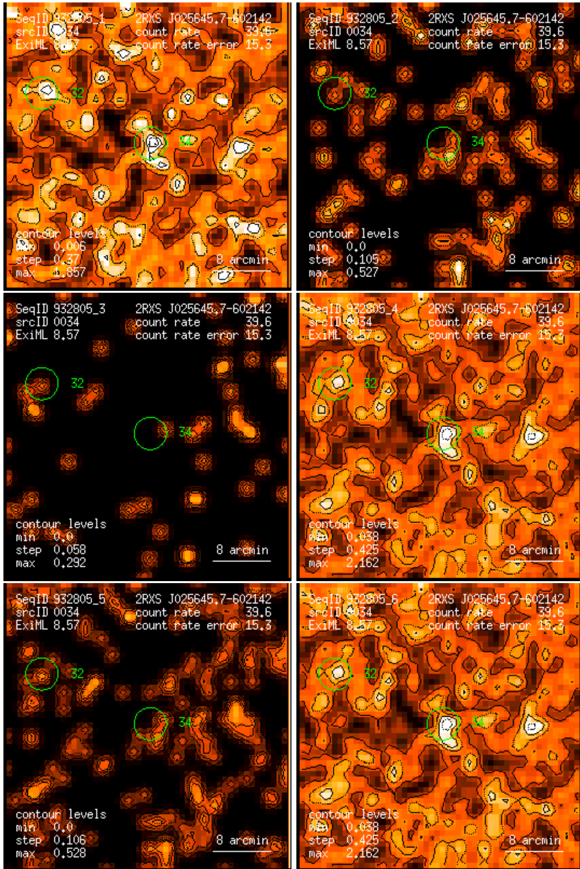
Figure 34: RASS 932805: detection 0034: band rate images, Gaussian filter: (1) PSPC channels 11 – 41, (2) 52 – 90, (3) 91 – 201, (4) 11 – 235, (5) 52 – 201, (6) 11 – 201. Broad band rates in counts/ks. Band rate contour levels in counts/ks/arcmin 2 .
