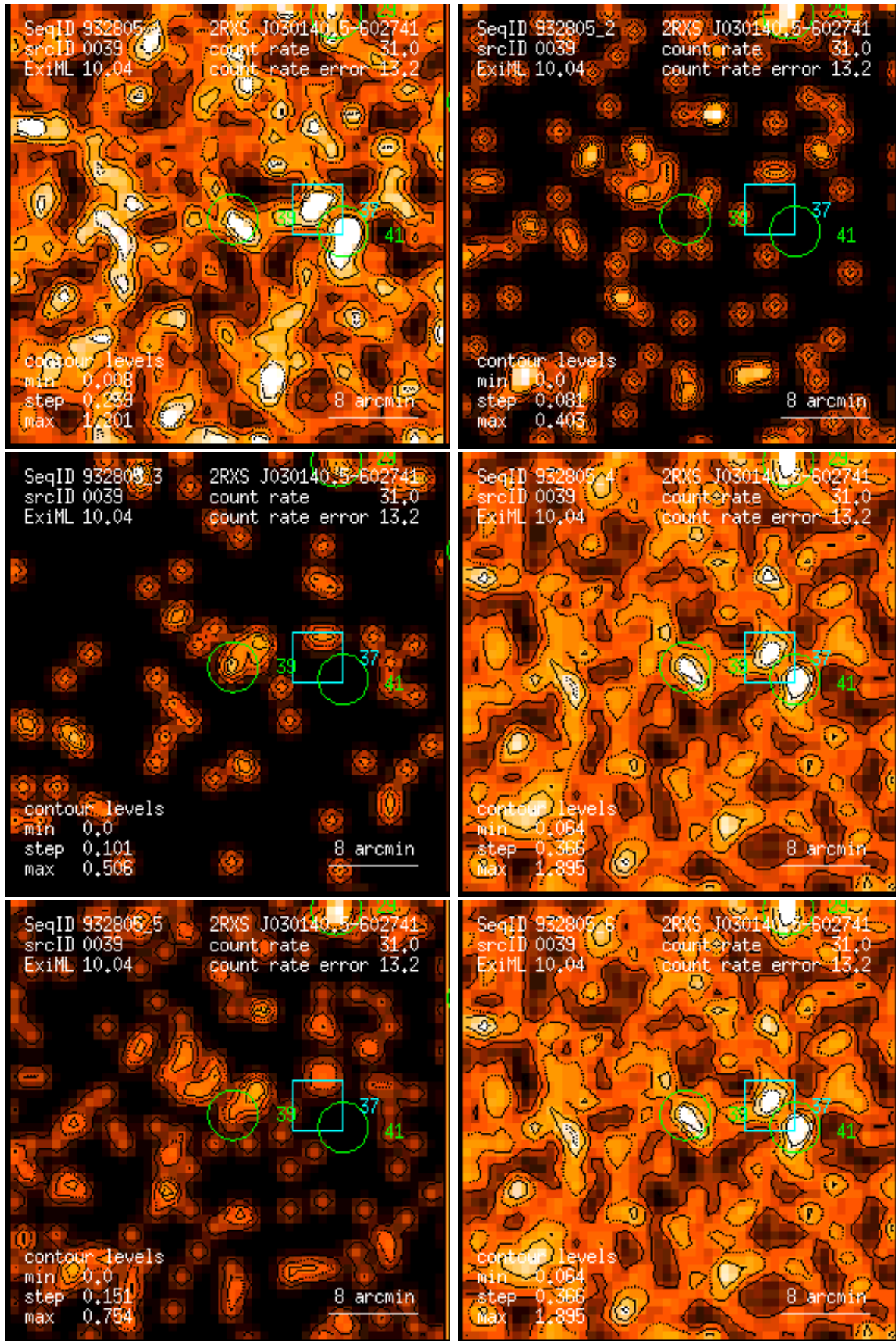
Figure 39: RASS 932805: detection 0039: band rate images, Gaussian filter: (1) PSPC channels 11 – 41, (2) 52 – 90, (3) 91 – 201, (4) 11 – 235, (5) 52 – 201, (6) 11 – 201. Broad band rates in counts/ks. Band rate contour levels in counts/ks/arcmin 2 .
